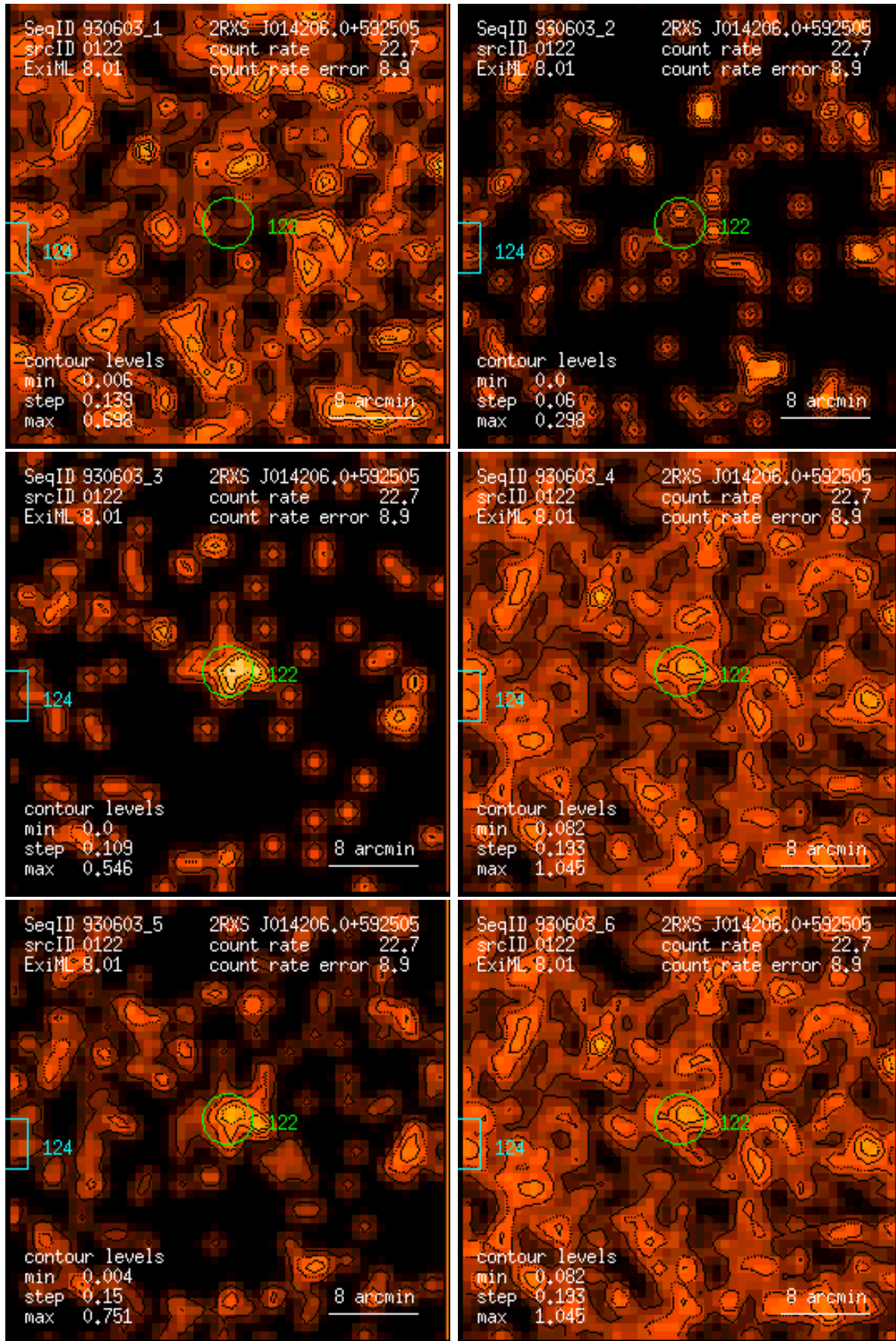
Figure 122: RASS 930603: detection 0122: band rate images, Gaussian filter: (1) PSPC channels 11 – 41, (2) 52 – 90, (3) 91 – 201, (4) 11 – 235, (5) 52 – 201, (6) 11 – 201. Broad band rates in counts/ks. Band rate contour levels in counts/ks/arcmin 2 .
