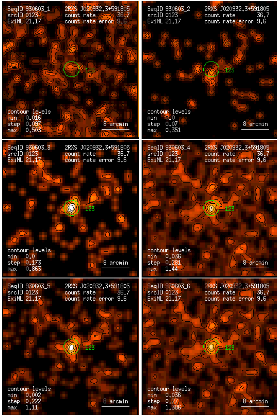
Figure 123: RASS 930603: detection 0123: band rate images, Gaussian filter: (1) PSPC channels 11 – 41, (2) 52 – 90, (3) 91 – 201, (4) 11 – 235, (5) 52 – 201, (6) 11 – 201. Broad band rates in counts/ks. Band rate contour levels in counts/ks/arcmin 2 .
