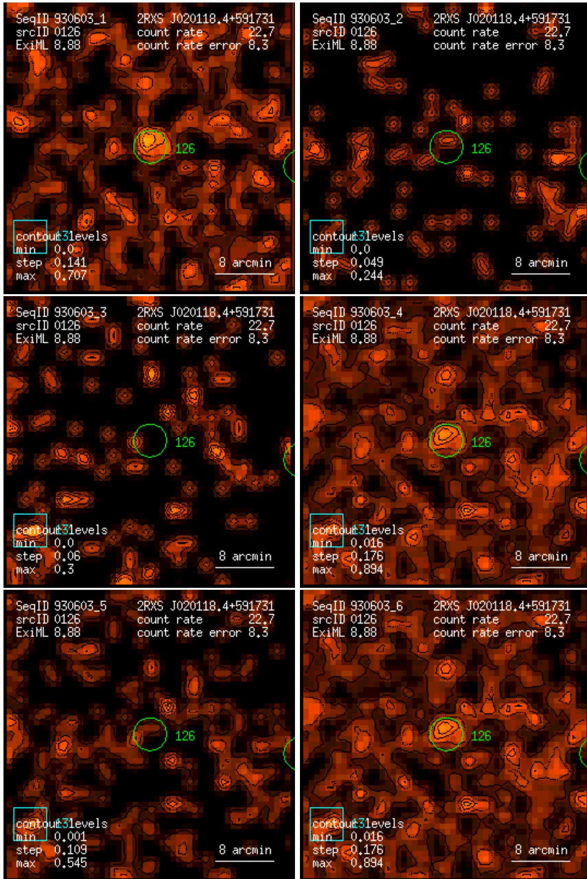
Figure 126: RASS 930603: detection 0126: band rate images, Gaussian filter: (1) PSPC channels 11 – 41, (2) 52 – 90, (3) 91 – 201, (4) 11 – 235, (5) 52 – 201, (6) 11 – 201. Broad band rates in counts/ks. Band rate contour levels in counts/ks/arcmin 2 .
