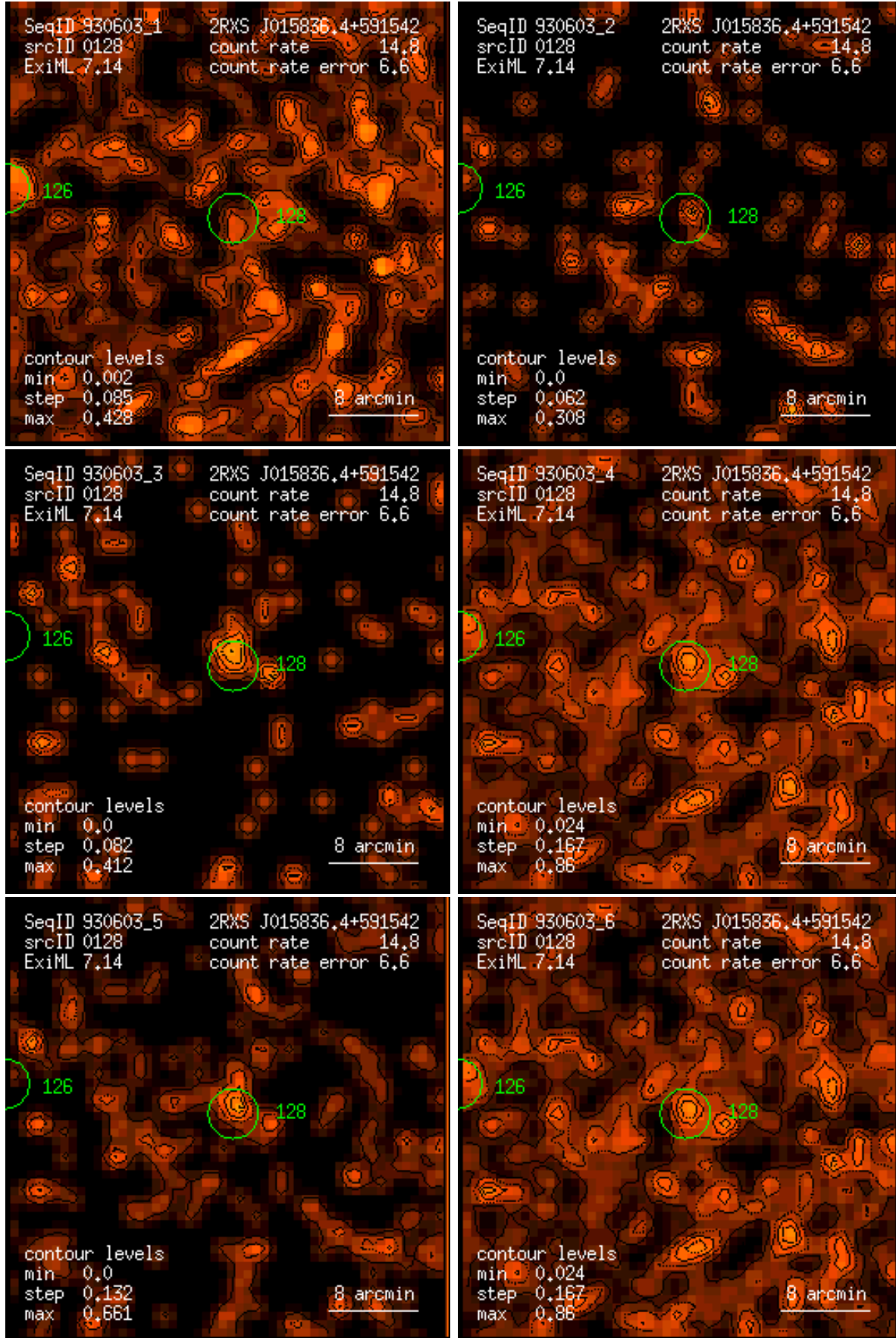
Figure 128: RASS 930603: detection 0128: band rate images, Gaussian filter: (1) PSPC channels 11 – 41, (2) 52 – 90, (3) 91 – 201, (4) 11 – 235, (5) 52 – 201, (6) 11 – 201. Broad band rates in counts/ks. Band rate contour levels in counts/ks/arcmin 2 .
