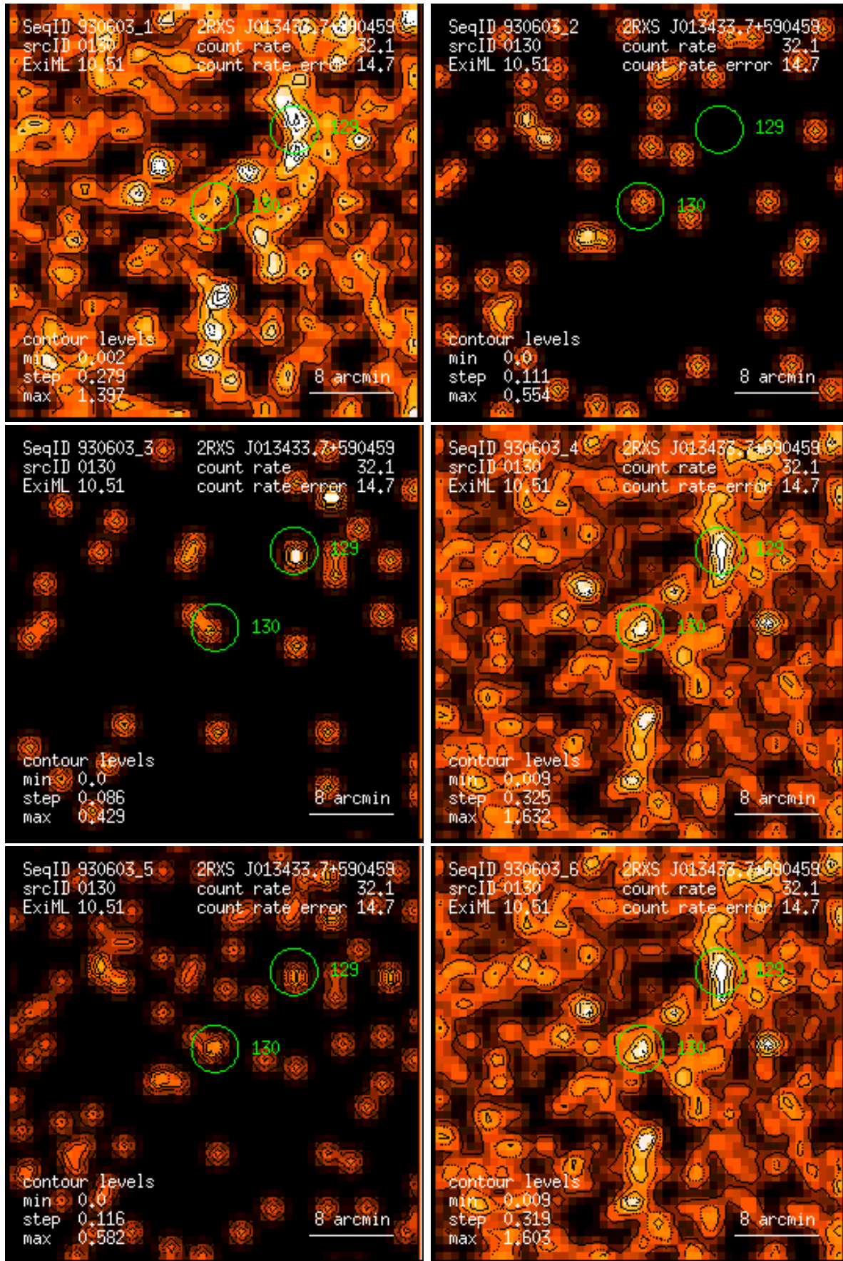
Figure 130: RASS 930603: detection 0130: band rate images, Gaussian filter: (1) PSPC channels 11 – 41, (2) 52 – 90, (3) 91 – 201, (4) 11 – 235, (5) 52 – 201, (6) 11 – 201. Broad band rates in counts/ks. Band rate contour levels in counts/ks/arcmin 2 .
