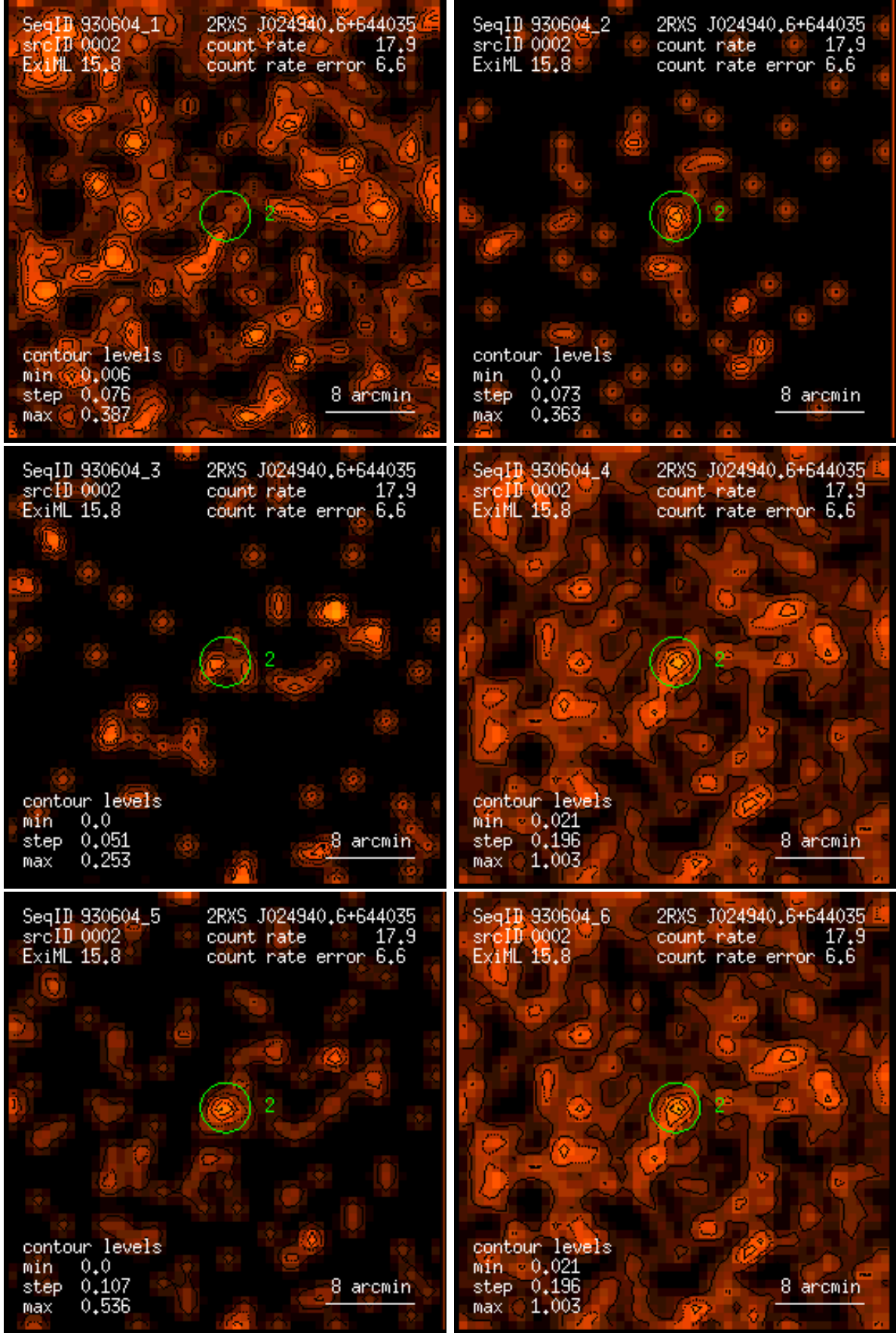
Figure 2: RASS 930604: detection 0002: band rate images, Gaussian filter: (1) PSPC channels 11 – 41, (2) 52 – 90, (3) 91 – 201, (4) 11 – 235, (5) 52 – 201, (6) 11 – 201. Broad band rates in counts/ks. Band rate contour levels in counts/ks/arcmin 2 .
