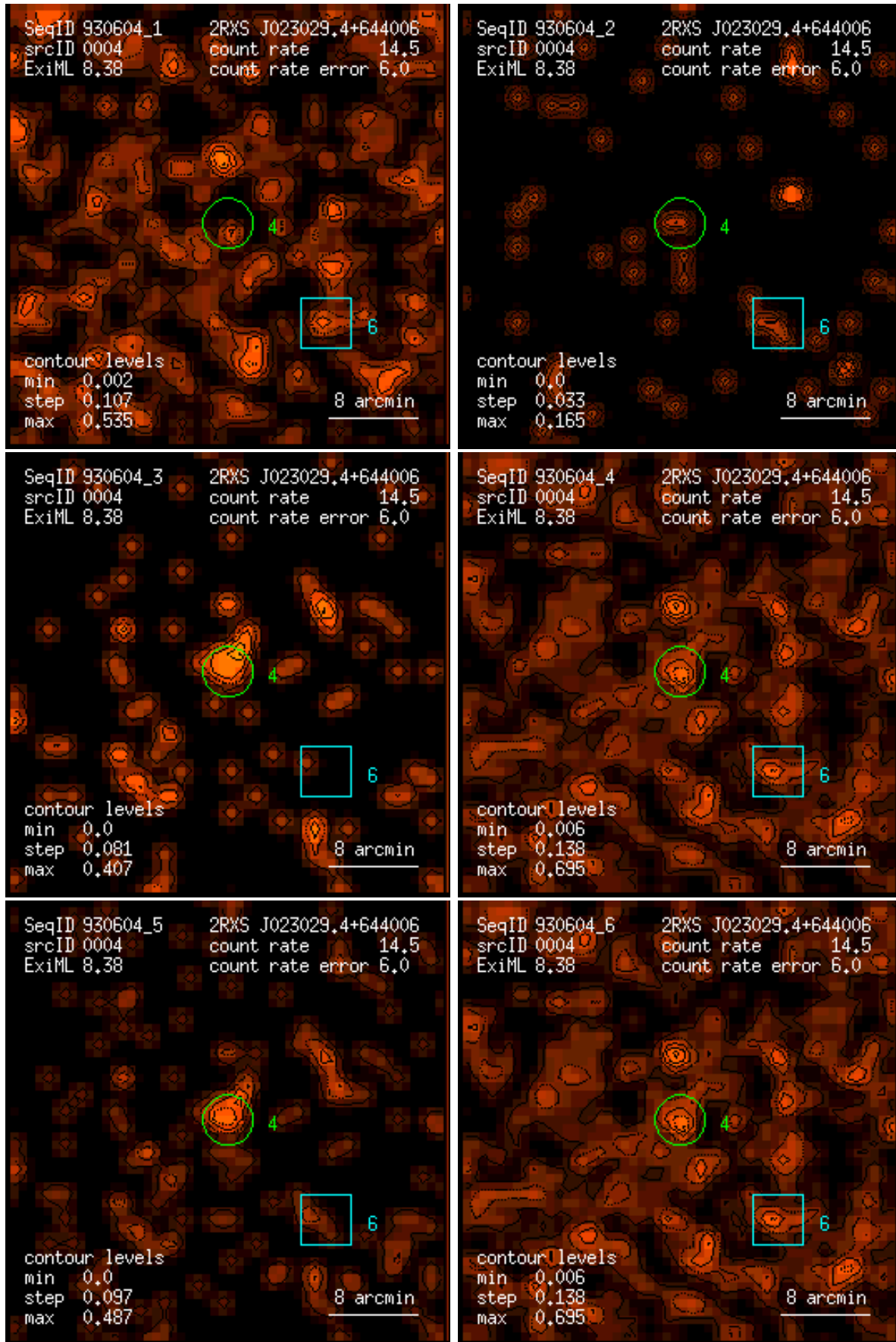
Figure 4: RASS 930604: detection 0004: band rate images, Gaussian filter: (1) PSPC channels 11 – 41, (2) 52 – 90, (3) 91 – 201, (4) 11 – 235, (5) 52 – 201, (6) 11 – 201. Broad band rates in counts/ks. Band rate contour levels in counts/ks/arcmin 2 .
