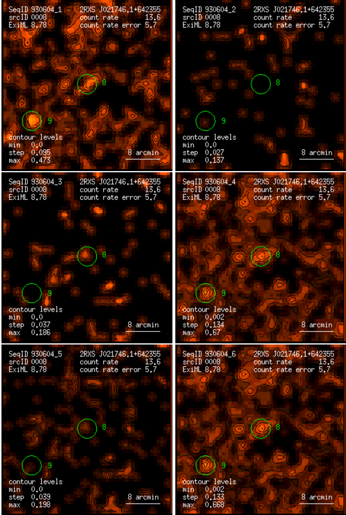
Figure 8: RASS 930604: detection 0008: band rate images, Gaussian filter: (1) PSPC channels 11 – 41, (2) 52 – 90, (3) 91 – 201, (4) 11 – 235, (5) 52 – 201, (6) 11 – 201. Broad band rates in counts/ks. Band rate contour levels in counts/ks/arcmin 2 .
