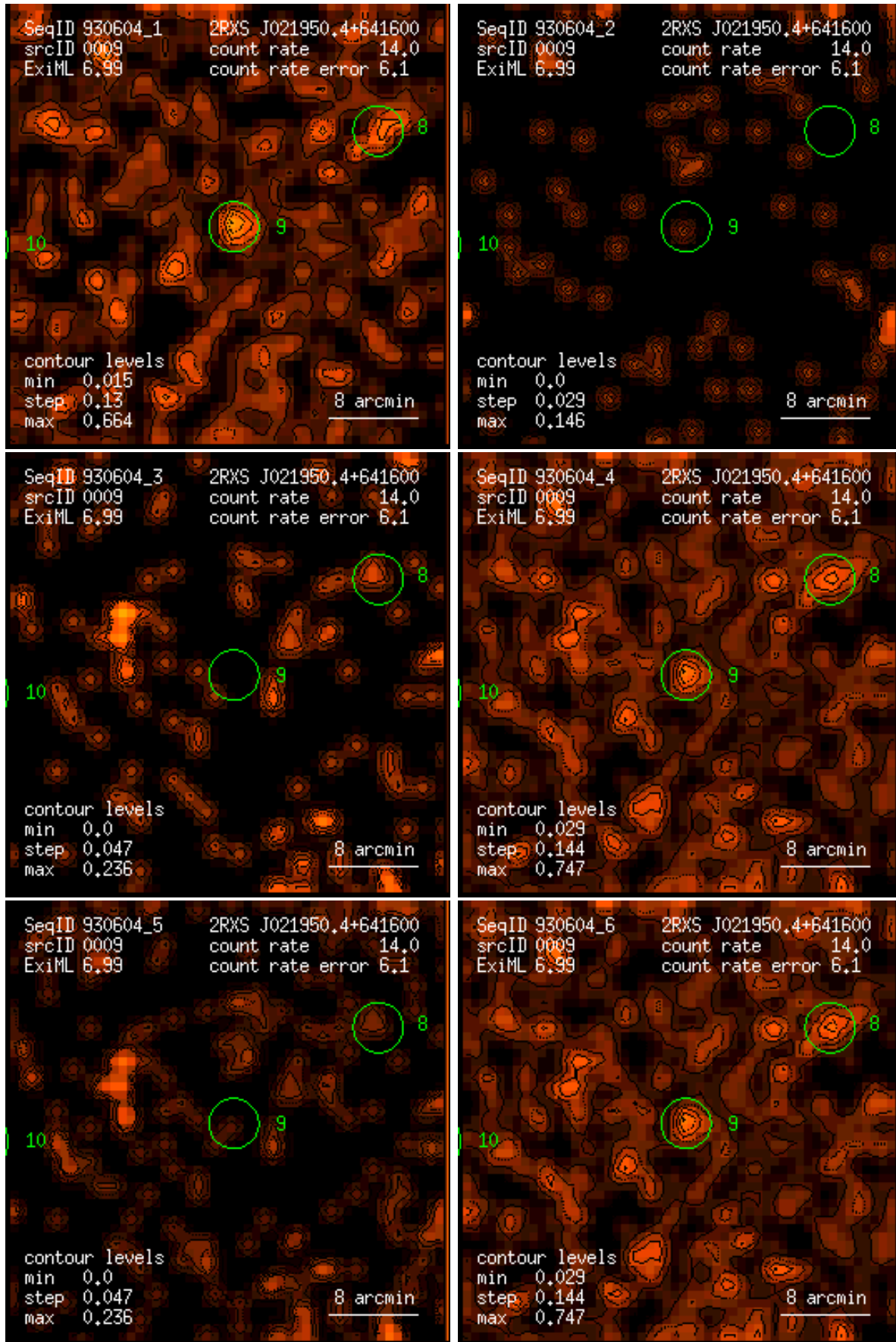
Figure 9: RASS 930604: detection 0009: band rate images, Gaussian filter: (1) PSPC channels 11 – 41, (2) 52 – 90, (3) 91 – 201, (4) 11 – 235, (5) 52 – 201, (6) 11 – 201. Broad band rates in counts/ks. Band rate contour levels in counts/ks/arcmin 2 .
