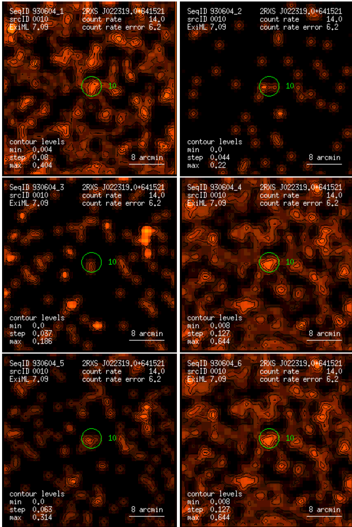
Figure 10: RASS 930604: detection 0010: band rate images, Gaussian filter: (1) PSPC channels 11 – 41, (2) 52 – 90, (3) 91 – 201, (4) 11 – 235, (5) 52 – 201, (6) 11 – 201. Broad band rates in counts/ks. Band rate contour levels in counts/ks/arcmin 2 .
