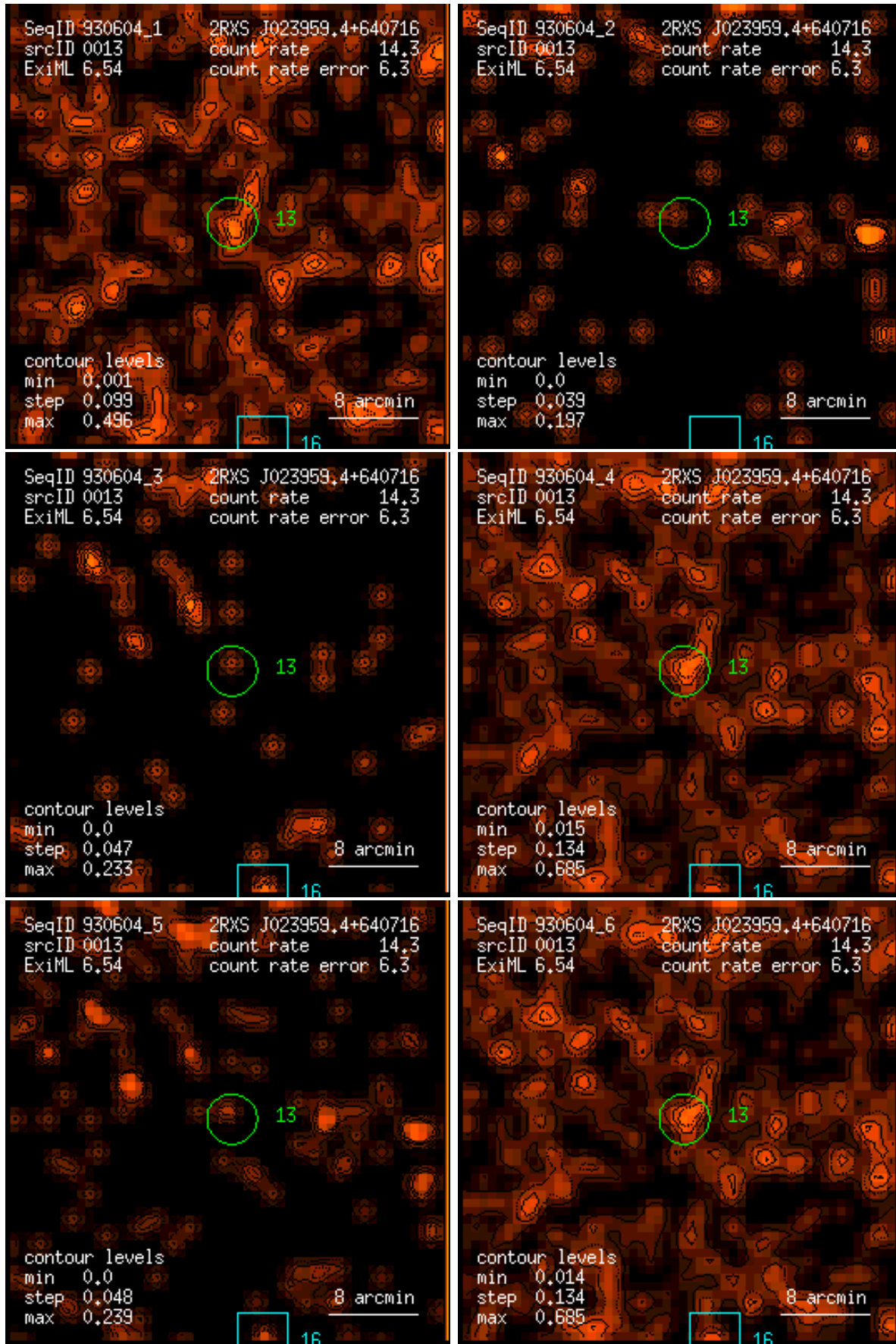
Figure 13: RASS 930604: detection 0013: band rate images, Gaussian filter: (1) PSPC channels 11 – 41, (2) 52 – 90, (3) 91 – 201, (4) 11 – 235, (5) 52 – 201, (6) 11 – 201. Broad band rates in counts/ks. Band rate contour levels in counts/ks/arcmin 2 .
