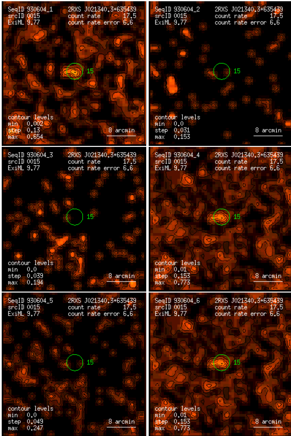
Figure 15: RASS 930604: detection 0015: band rate images, Gaussian filter: (1) PSPC channels 11 – 41, (2) 52 – 90, (3) 91 – 201, (4) 11 – 235, (5) 52 – 201, (6) 11 – 201. Broad band rates in counts/ks. Band rate contour levels in counts/ks/arcmin 2 .
