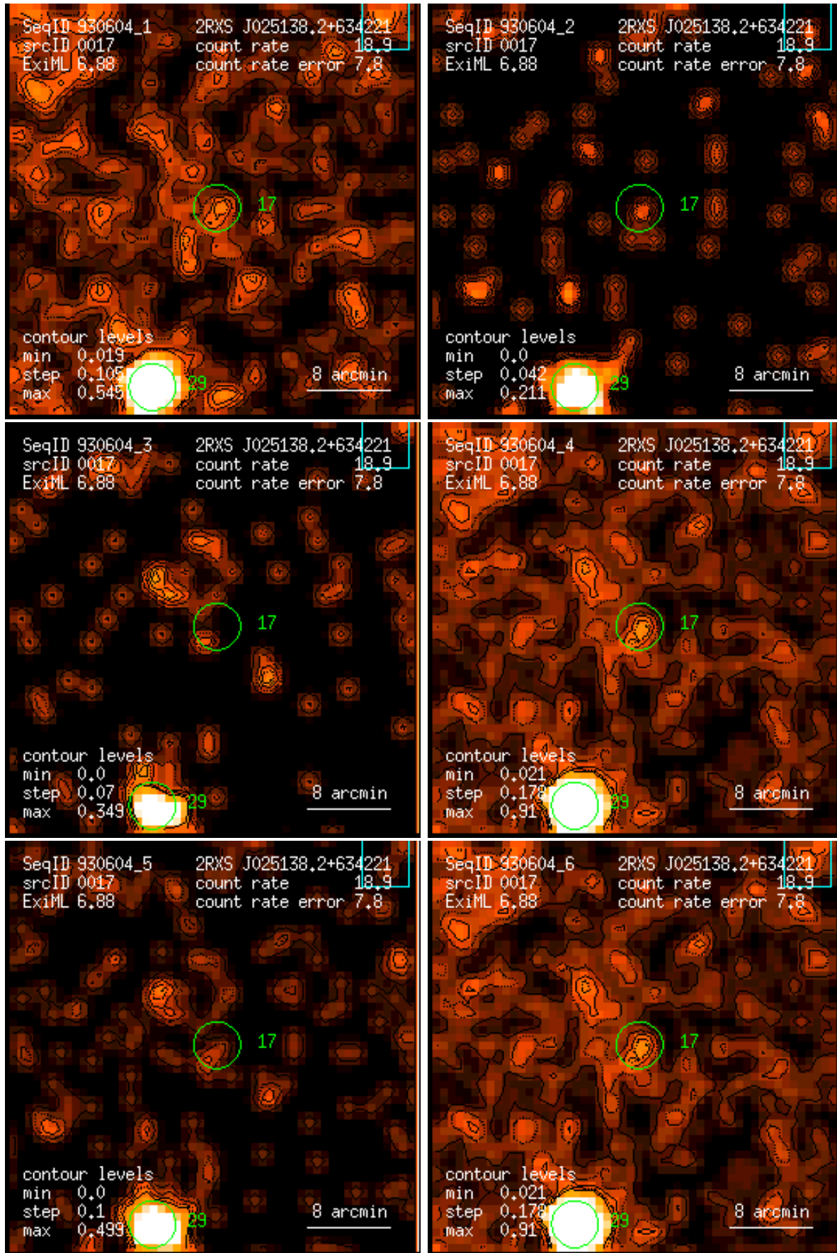
Figure 17: RASS 930604: detection 0017: band rate images, Gaussian filter: (1) PSPC channels 11 – 41, (2) 52 – 90, (3) 91 – 201, (4) 11 – 235, (5) 52 – 201, (6) 11 – 201. Broad band rates in counts/ks. Band rate contour levels in counts/ks/arcmin 2 .
