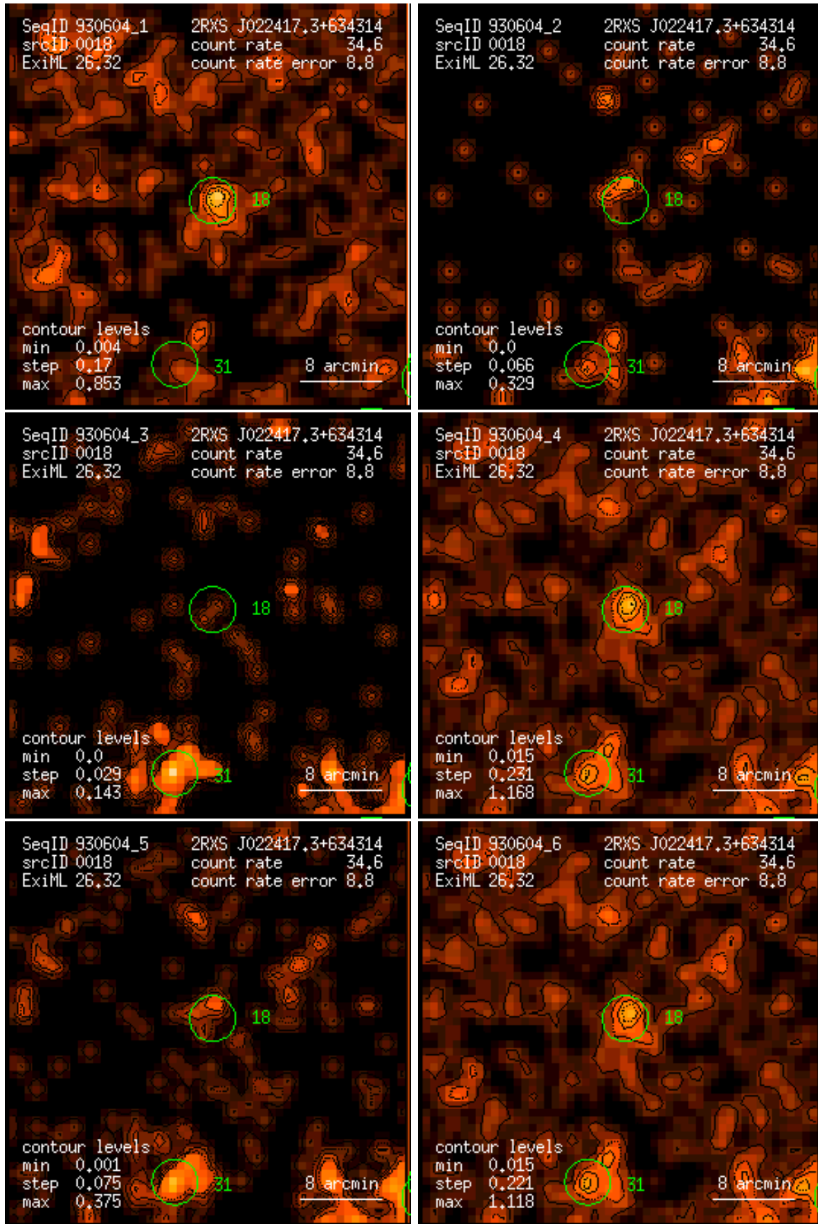
Figure 18: RASS 930604: detection 0018: band rate images, Gaussian filter: (1) PSPC channels 11 – 41, (2) 52 – 90, (3) 91 – 201, (4) 11 – 235, (5) 52 – 201, (6) 11 – 201. Broad band rates in counts/ks. Band rate contour levels in counts/ks/arcmin 2 .
