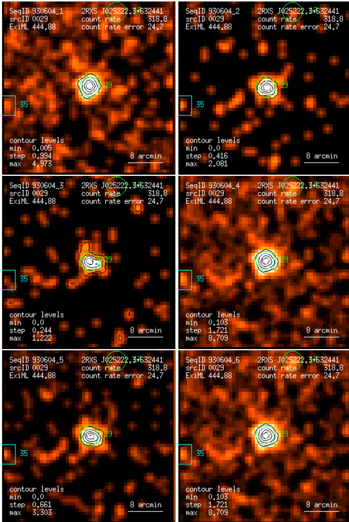
Figure 29: RASS 930604: detection 0029: band rate images, Gaussian filter: (1) PSPC channels 11 – 41, (2) 52 – 90, (3) 91 – 201, (4) 11 – 235, (5) 52 – 201, (6) 11 – 201. Broad band rates in counts/ks. Band rate contour levels in counts/ks/arcmin 2 .
