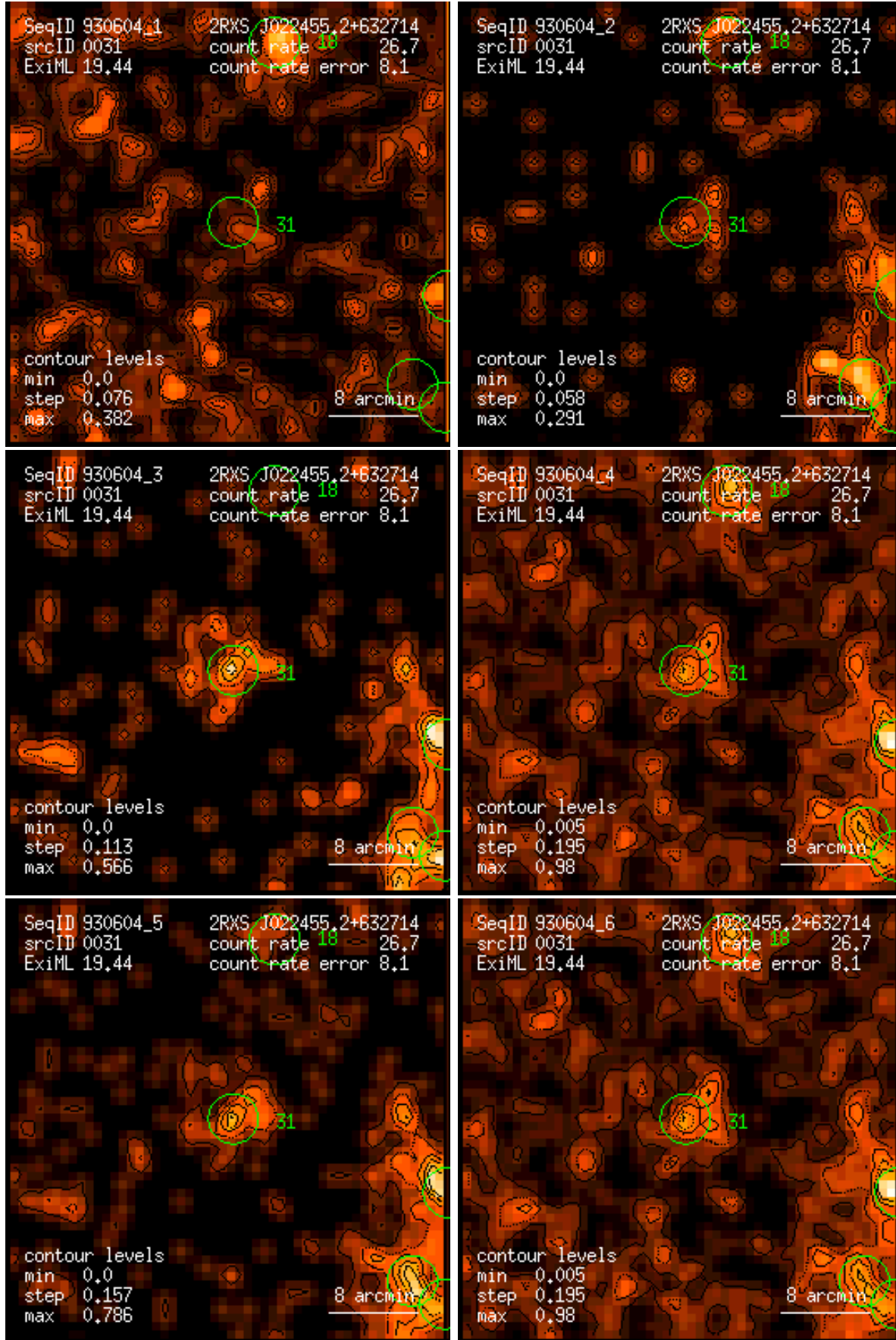
Figure 31: RASS 930604: detection 0031: band rate images, Gaussian filter: (1) PSPC channels 11 – 41, (2) 52 – 90, (3) 91 – 201, (4) 11 – 235, (5) 52 – 201, (6) 11 – 201. Broad band rates in counts/ks. Band rate contour levels in counts/ks/arcmin 2 .
