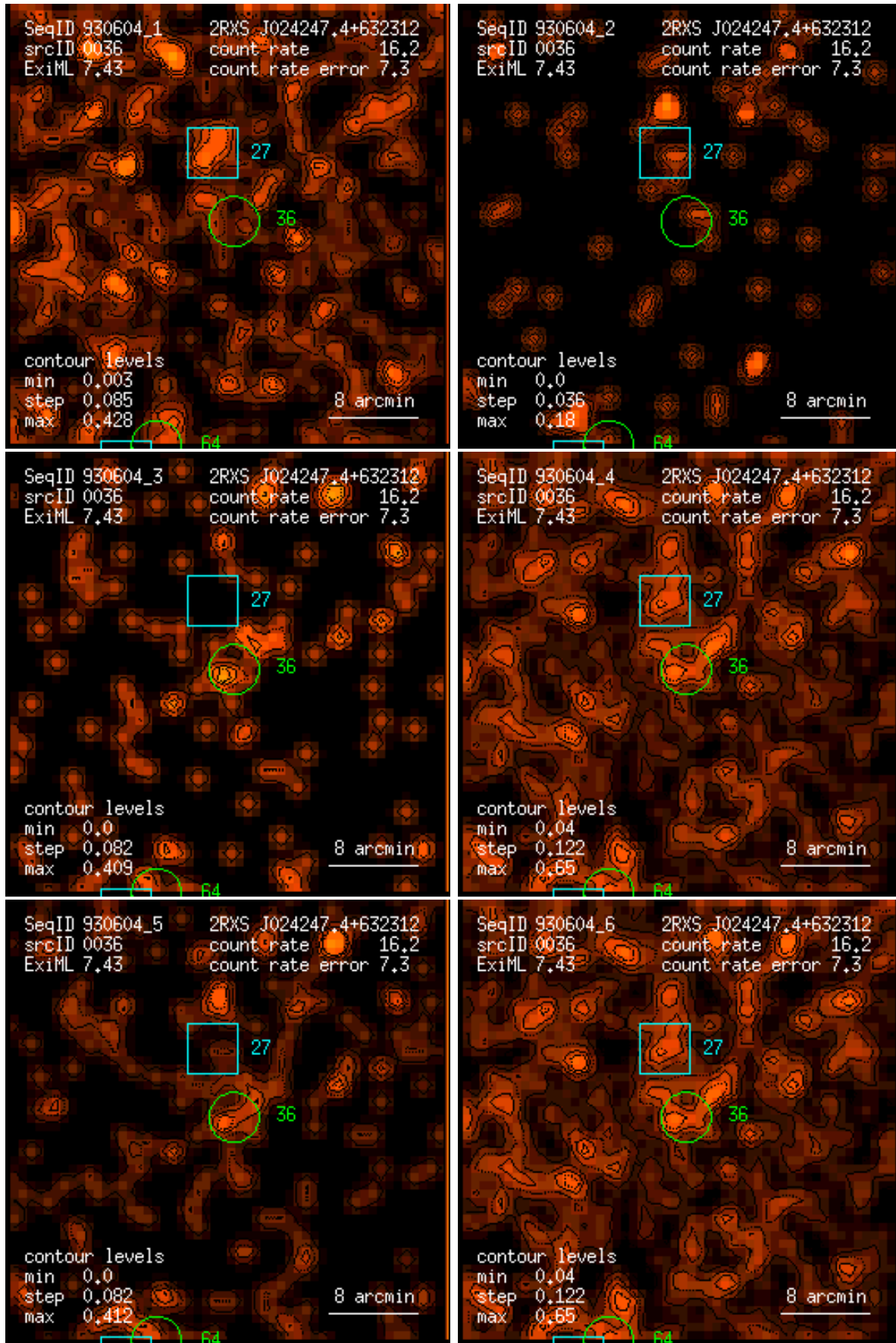
Figure 36: RASS 930604: detection 0036: band rate images, Gaussian filter: (1) PSPC channels 11 – 41, (2) 52 – 90, (3) 91 – 201, (4) 11 – 235, (5) 52 – 201, (6) 11 – 201. Broad band rates in counts/ks. Band rate contour levels in counts/ks/arcmin 2 .
