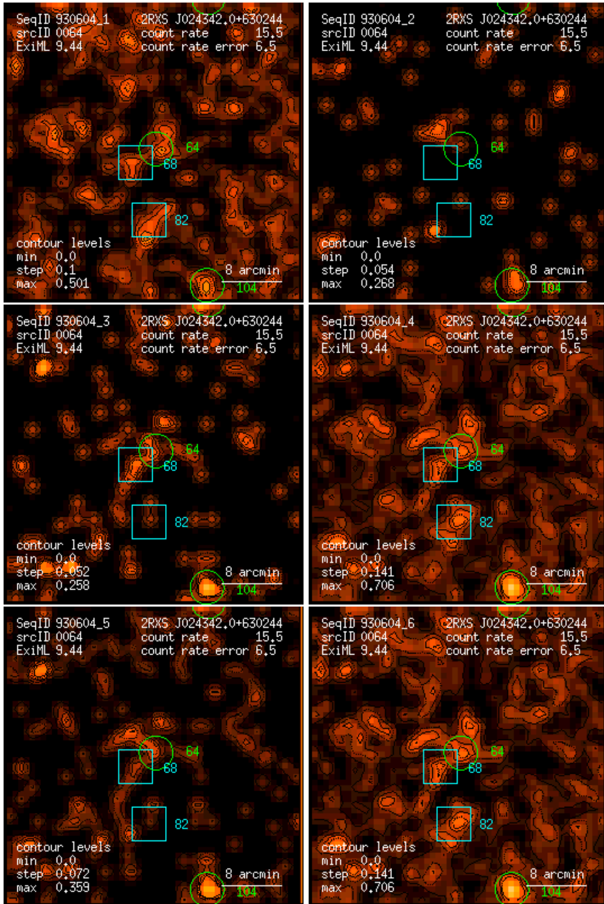
Figure 64: RASS 930604: detection 0064: band rate images, Gaussian filter: (1) PSPC channels 11 – 41, (2) 52 – 90, (3) 91 – 201, (4) 11 – 235, (5) 52 – 201, (6) 11 – 201. Broad band rates in counts/ks. Band rate contour levels in counts/ks/arcmin 2 .
