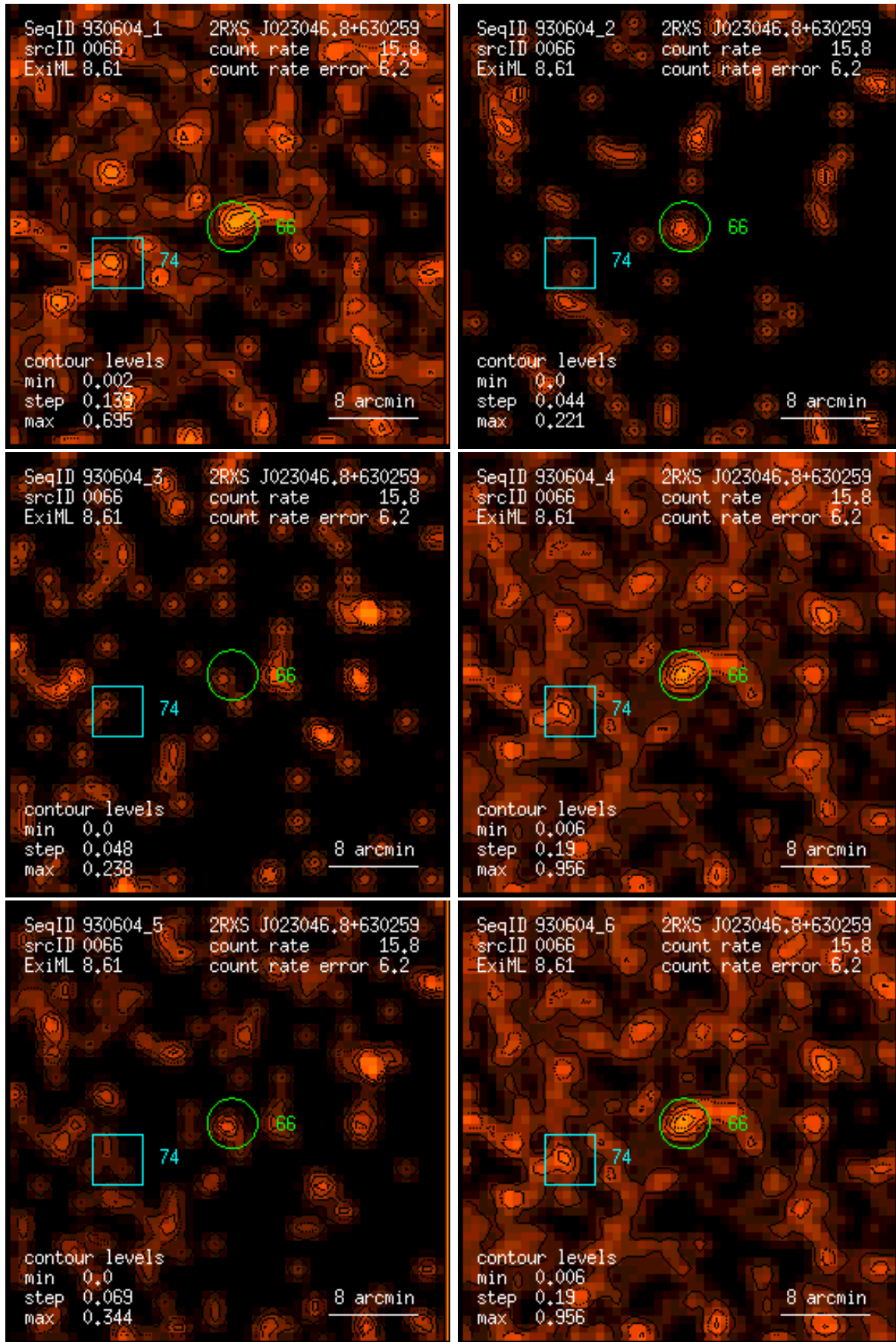
Figure 66: RASS 930604: detection 0066: band rate images, Gaussian filter: (1) PSPC channels 11 – 41, (2) 52 – 90, (3) 91 – 201, (4) 11 – 235, (5) 52 – 201, (6) 11 – 201. Broad band rates in counts/ks. Band rate contour levels in counts/ks/arcmin 2 .
