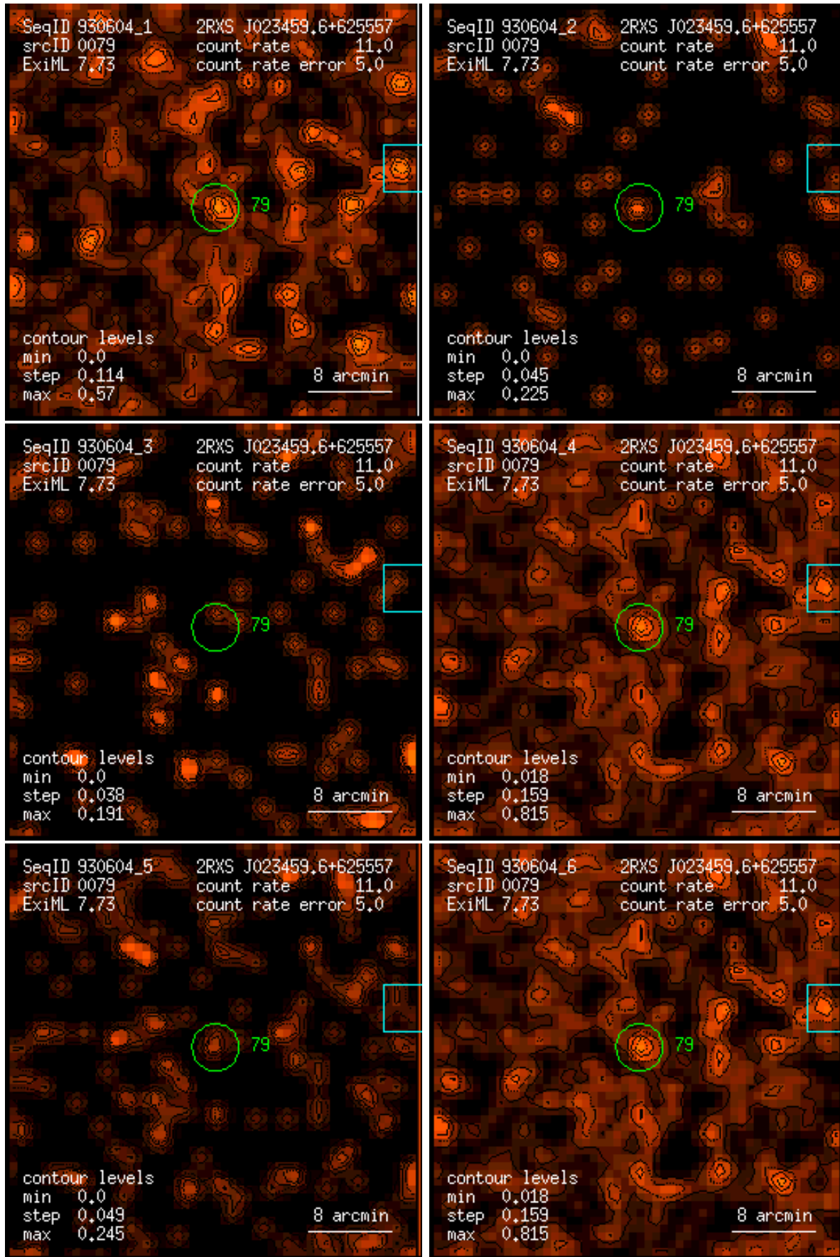
Figure 79: RASS 930604: detection 0079: band rate images, Gaussian filter: (1) PSPC channels 11 – 41, (2) 52 – 90, (3) 91 – 201, (4) 11 – 235, (5) 52 – 201, (6) 11 – 201. Broad band rates in counts/ks. Band rate contour levels in counts/ks/arcmin 2 .
