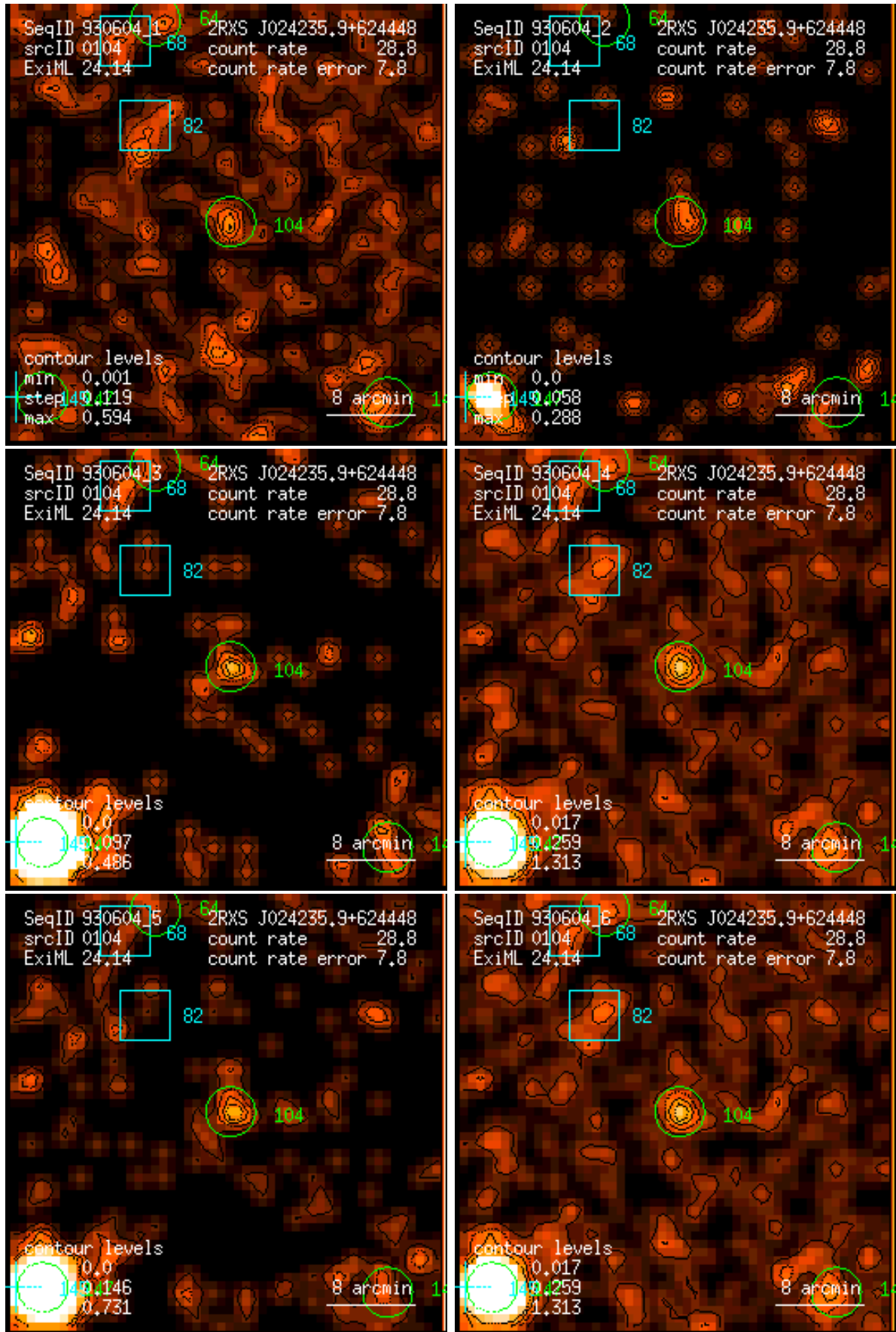
Figure 104: RASS 930604: detection 0104: band rate images, Gaussian filter: (1) PSPC channels 11 – 41, (2) 52 – 90, (3) 91 – 201, (4) 11 – 235, (5) 52 – 201, (6) 11 – 201. Broad band rates in counts/ks. Band rate contour levels in counts/ks/arcmin 2 .
