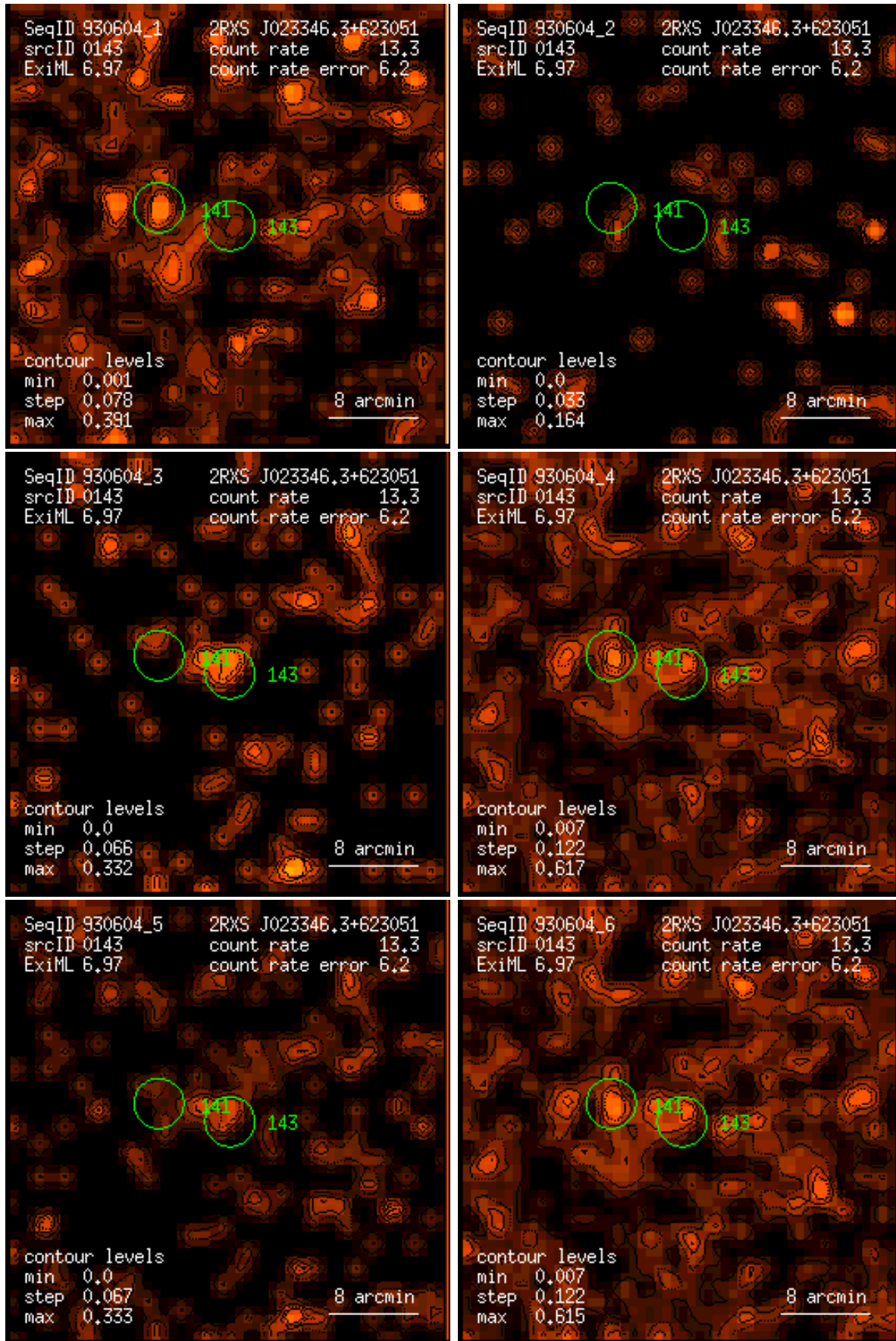
Figure 143: RASS 930604: detection 0143: band rate images, Gaussian filter: (1) PSPC channels 11 – 41, (2) 52 – 90, (3) 91 – 201, (4) 11 – 235, (5) 52 – 201, (6) 11 – 201. Broad band rates in counts/ks. Band rate contour levels in counts/ks/arcmin 2 .
