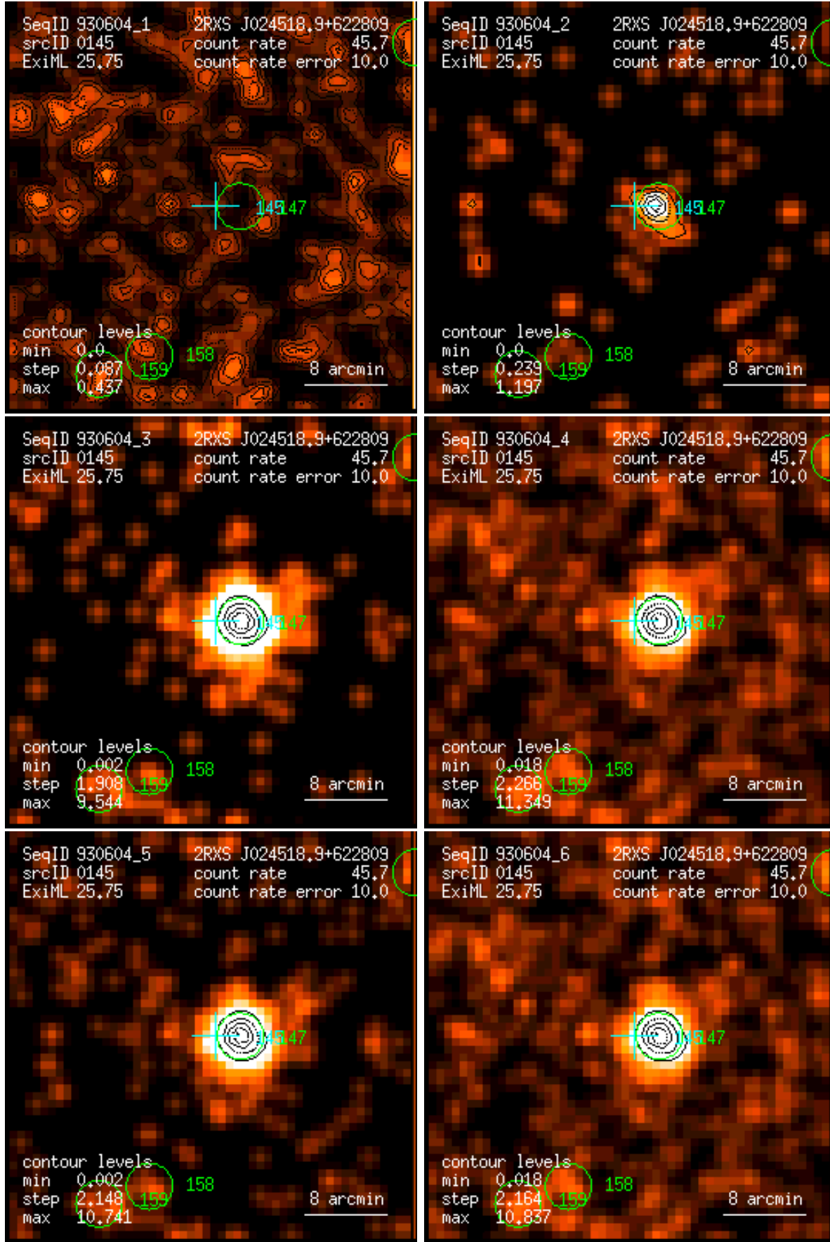
Figure 145: RASS 930604: detection 0145: band rate images, Gaussian filter: (1) PSPC channels 11 – 41, (2) 52 – 90, (3) 91 – 201, (4) 11 – 235, (5) 52 – 201, (6) 11 – 201. Broad band rates in counts/ks. Band rate contour levels in counts/ks/arcmin 2 .
