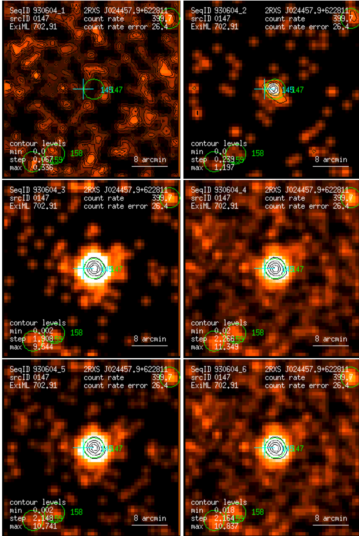
Figure 147: RASS 930604: detection 0147: band rate images, Gaussian filter: (1) PSPC channels 11 – 41, (2) 52 – 90, (3) 91 – 201, (4) 11 – 235, (5) 52 – 201, (6) 11 – 201. Broad band rates in counts/ks. Band rate contour levels in counts/ks/arcmin 2 .
