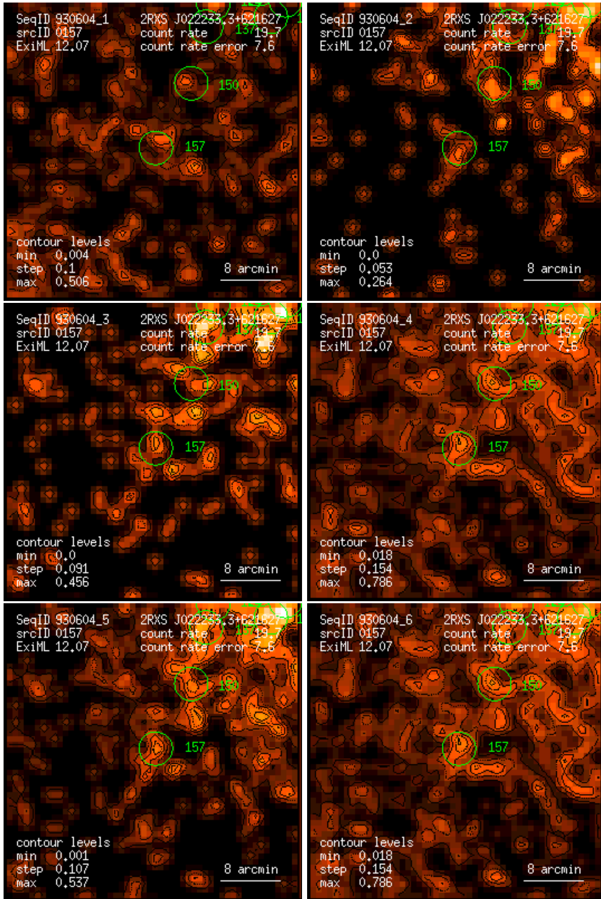
Figure 157: RASS 930604: detection 0157: band rate images, Gaussian filter: (1) PSPC channels 11 – 41, (2) 52 – 90, (3) 91 – 201, (4) 11 – 235, (5) 52 – 201, (6) 11 – 201. Broad band rates in counts/ks. Band rate contour levels in counts/ks/arcmin 2 .
