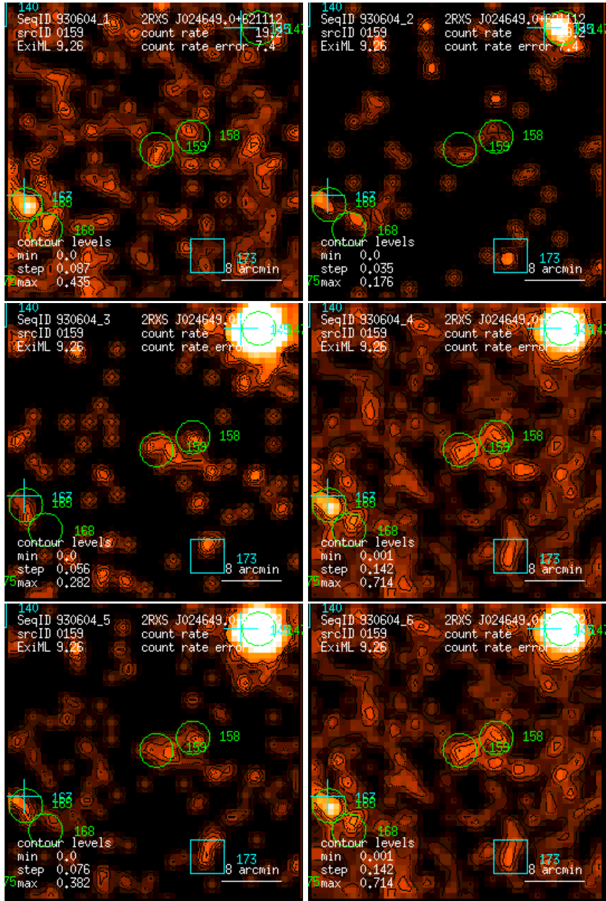
Figure 159: RASS 930604: detection 0159: band rate images, Gaussian filter: (1) PSPC channels 11 – 41, (2) 52 – 90, (3) 91 – 201, (4) 11 – 235, (5) 52 – 201, (6) 11 – 201. Broad band rates in counts/ks. Band rate contour levels in counts/ks/arcmin 2 .
