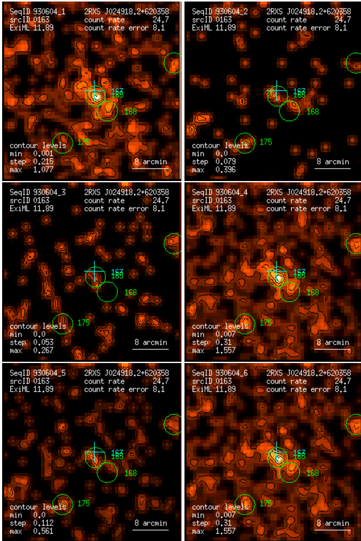
Figure 163: RASS 930604: detection 0163: band rate images, Gaussian filter: (1) PSPC channels 11 – 41, (2) 52 – 90, (3) 91 – 201, (4) 11 – 235, (5) 52 – 201, (6) 11 – 201. Broad band rates in counts/ks. Band rate contour levels in counts/ks/arcmin 2 .
