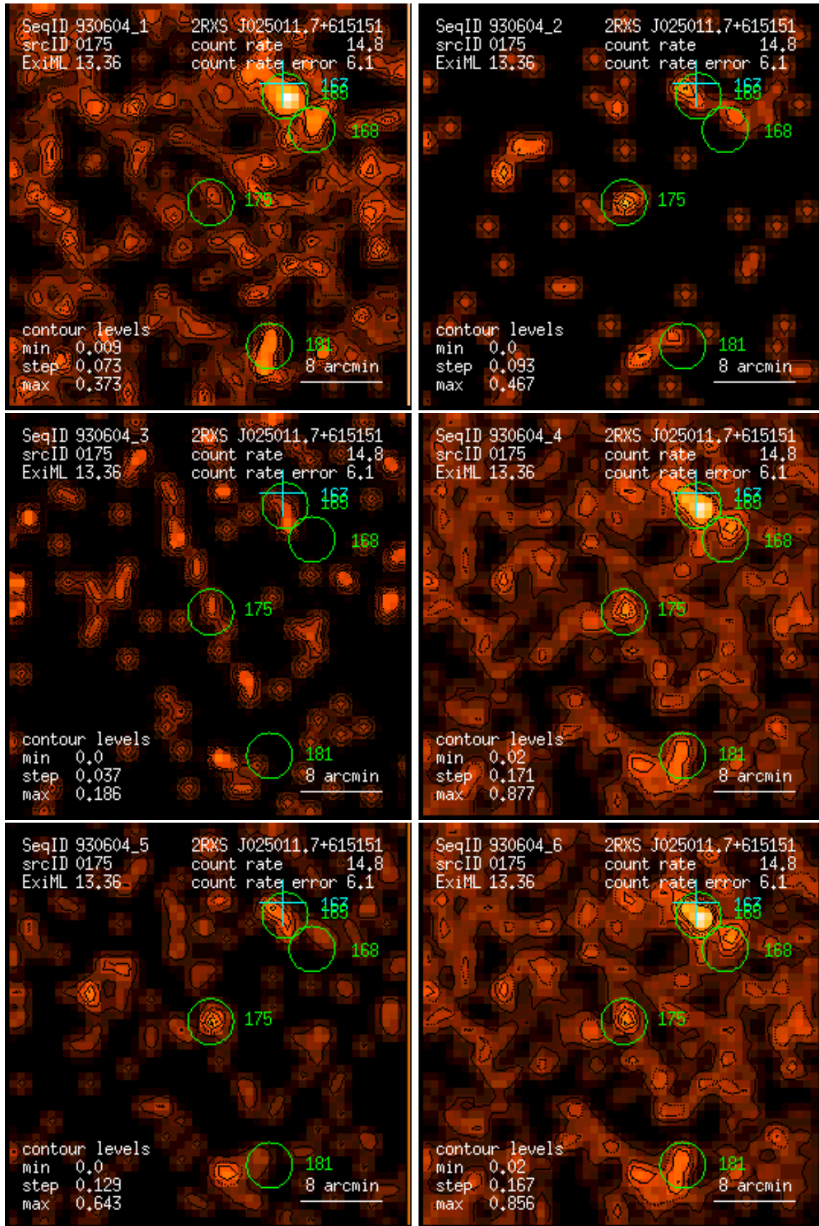
Figure 175: RASS 930604: detection 0175: band rate images, Gaussian filter: (1) PSPC channels 11 – 41, (2) 52 – 90, (3) 91 – 201, (4) 11 – 235, (5) 52 – 201, (6) 11 – 201. Broad band rates in counts/ks. Band rate contour levels in counts/ks/arcmin 2 .
