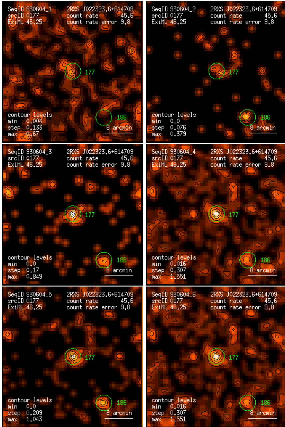
Figure 177: RASS 930604: detection 0177: band rate images, Gaussian filter: (1) PSPC channels 11 – 41, (2) 52 – 90, (3) 91 – 201, (4) 11 – 235, (5) 52 – 201, (6) 11 – 201. Broad band rates in counts/ks. Band rate contour levels in counts/ks/arcmin 2 .
