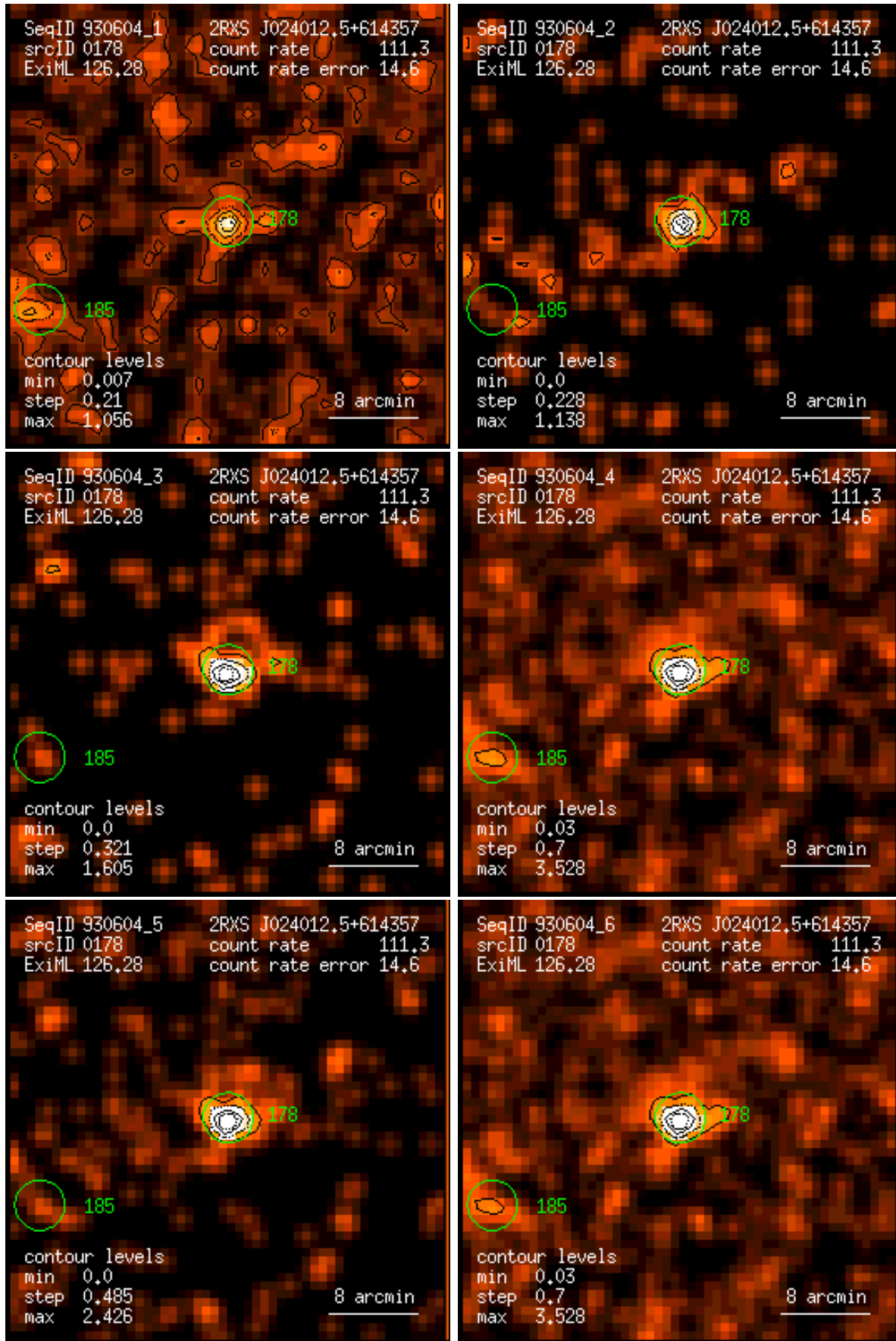
Figure 178: RASS 930604: detection 0178: band rate images, Gaussian filter: (1) PSPC channels 11 – 41, (2) 52 – 90, (3) 91 – 201, (4) 11 – 235, (5) 52 – 201, (6) 11 – 201. Broad band rates in counts/ks. Band rate contour levels in counts/ks/arcmin 2 .
