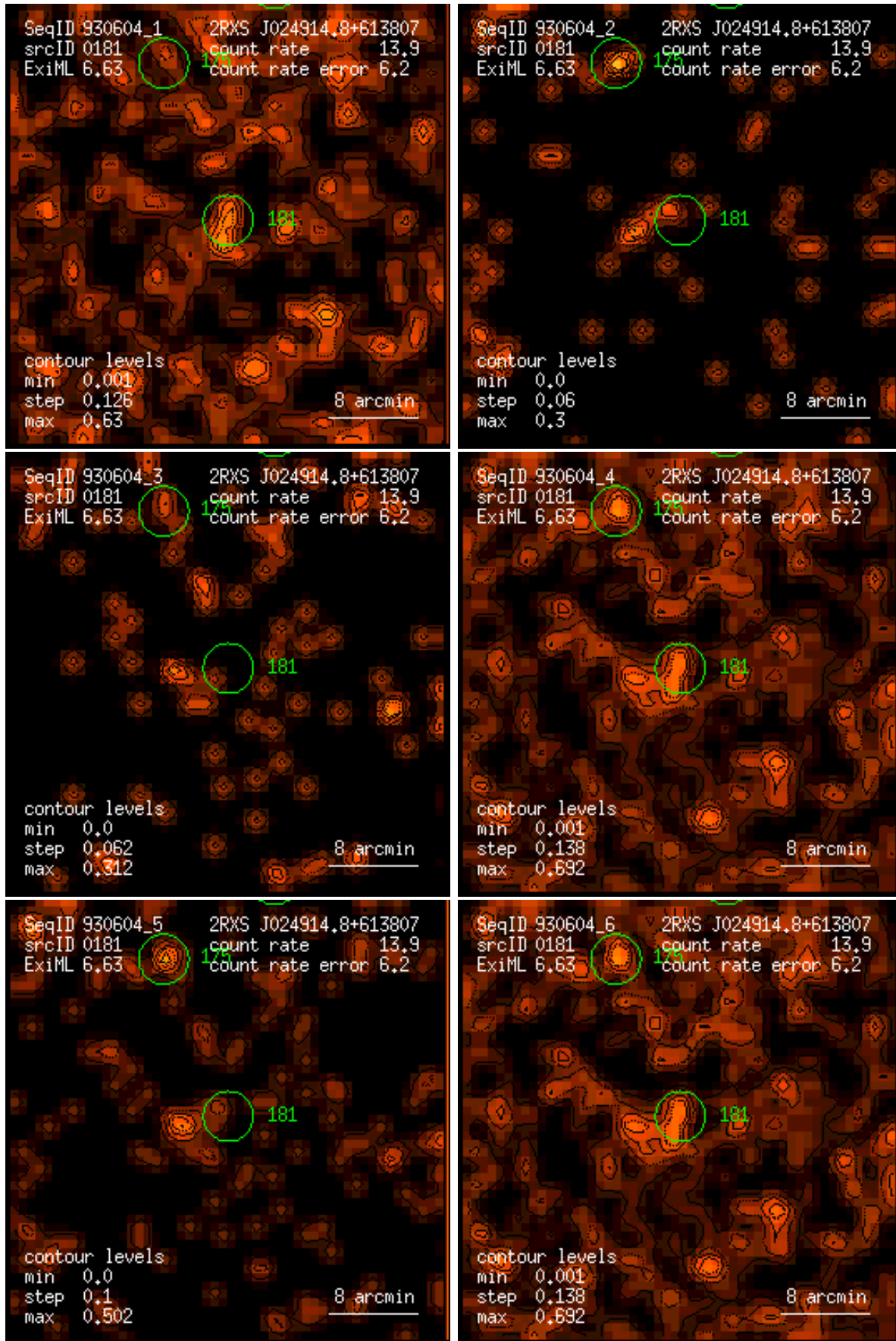
Figure 181: RASS 930604: detection 0181: band rate images, Gaussian filter: (1) PSPC channels 11 – 41, (2) 52 – 90, (3) 91 – 201, (4) 11 – 235, (5) 52 – 201, (6) 11 – 201. Broad band rates in counts/ks. Band rate contour levels in counts/ks/arcmin 2 .
