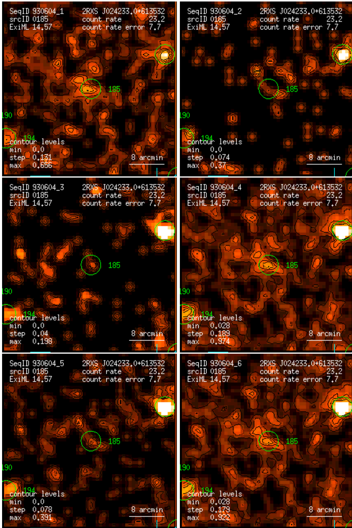
Figure 185: RASS 930604: detection 0185: band rate images, Gaussian filter: (1) PSPC channels 11 – 41, (2) 52 – 90, (3) 91 – 201, (4) 11 – 235, (5) 52 – 201, (6) 11 – 201. Broad band rates in counts/ks. Band rate contour levels in counts/ks/arcmin 2 .
