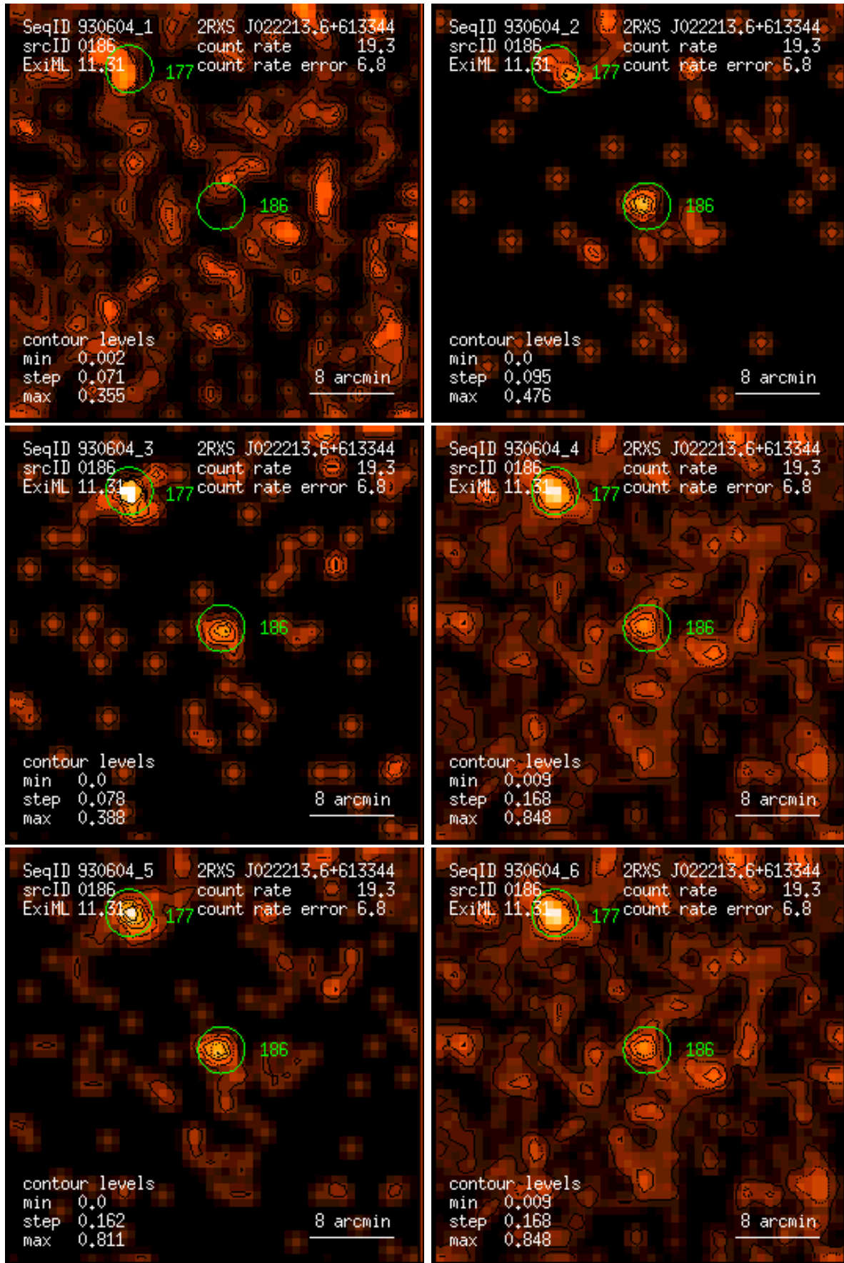
Figure 186: RASS 930604: detection 0186: band rate images, Gaussian filter: (1) PSPC channels 11 – 41, (2) 52 – 90, (3) 91 – 201, (4) 11 – 235, (5) 52 – 201, (6) 11 – 201. Broad band rates in counts/ks. Band rate contour levels in counts/ks/arcmin 2 .
