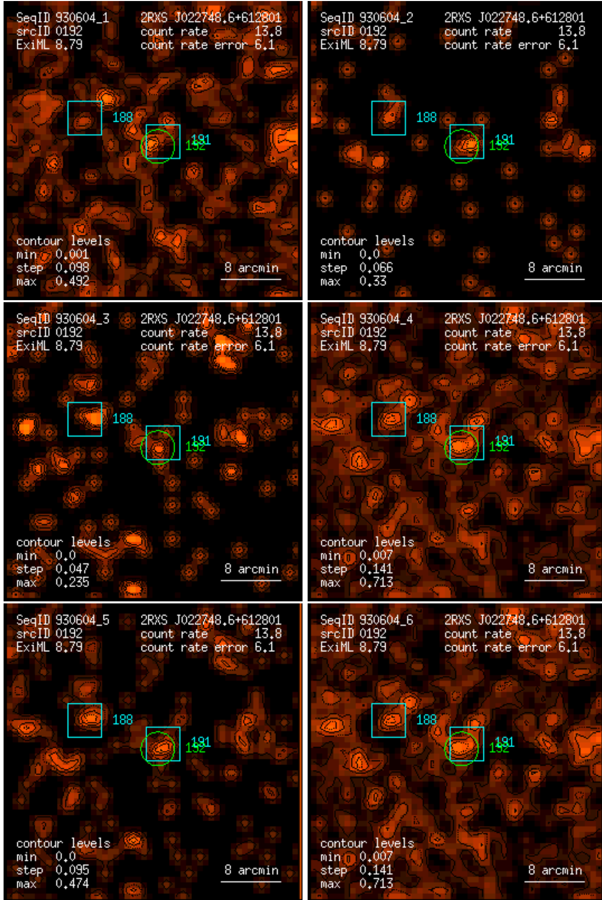
Figure 192: RASS 930604: detection 0192: band rate images, Gaussian filter: (1) PSPC channels 11 – 41, (2) 52 – 90, (3) 91 – 201, (4) 11 – 235, (5) 52 – 201, (6) 11 – 201. Broad band rates in counts/ks. Band rate contour levels in counts/ks/arcmin 2 .
