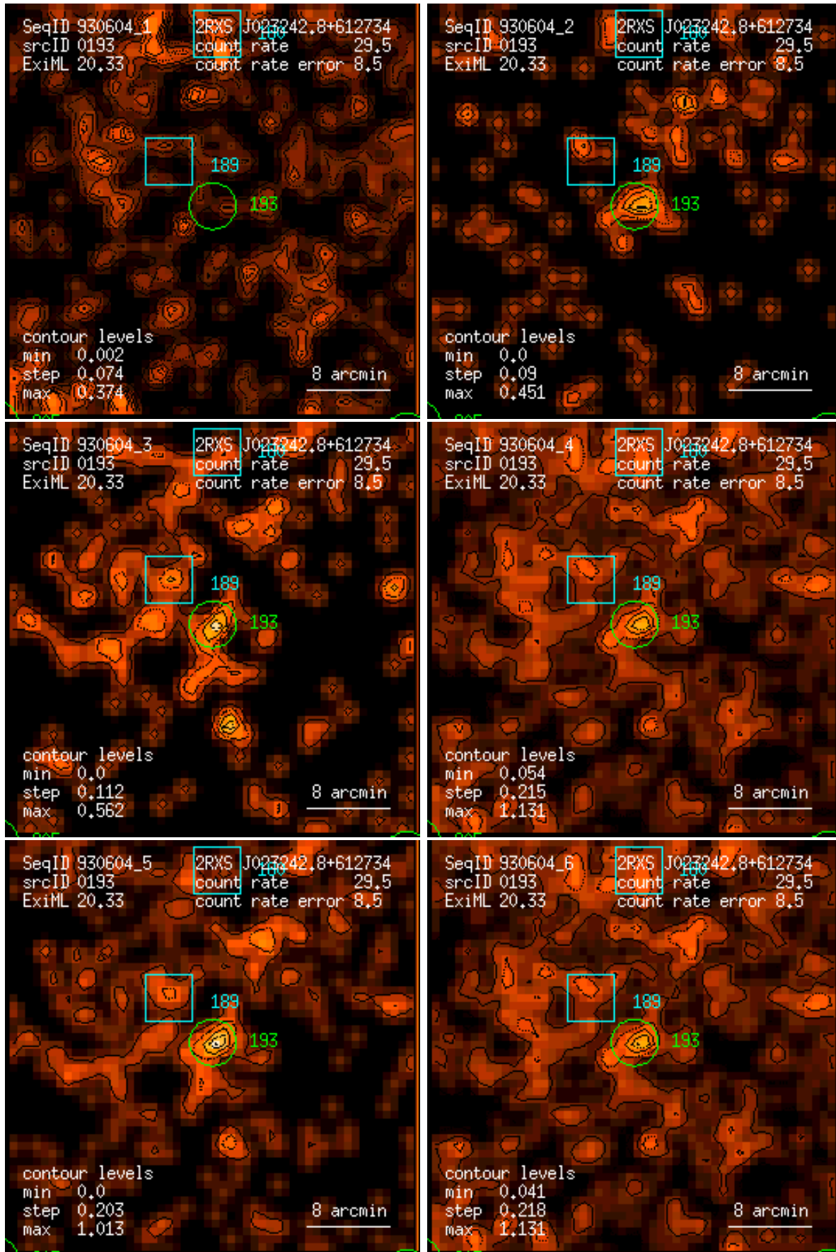
Figure 193: RASS 930604: detection 0193: band rate images, Gaussian filter: (1) PSPC channels 11 – 41, (2) 52 – 90, (3) 91 – 201, (4) 11 – 235, (5) 52 – 201, (6) 11 – 201. Broad band rates in counts/ks. Band rate contour levels in counts/ks/arcmin 2 .
