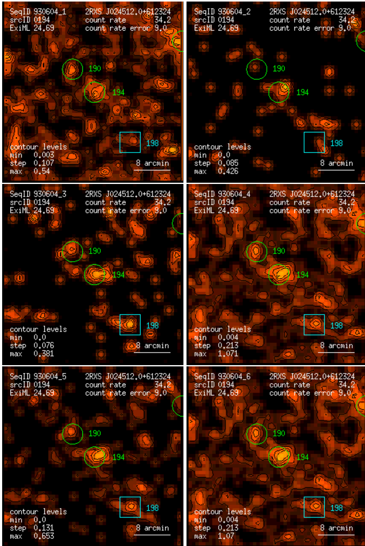
Figure 194: RASS 930604: detection 0194: band rate images, Gaussian filter: (1) PSPC channels 11 – 41, (2) 52 – 90, (3) 91 – 201, (4) 11 – 235, (5) 52 – 201, (6) 11 – 201. Broad band rates in counts/ks. Band rate contour levels in counts/ks/arcmin 2 .
