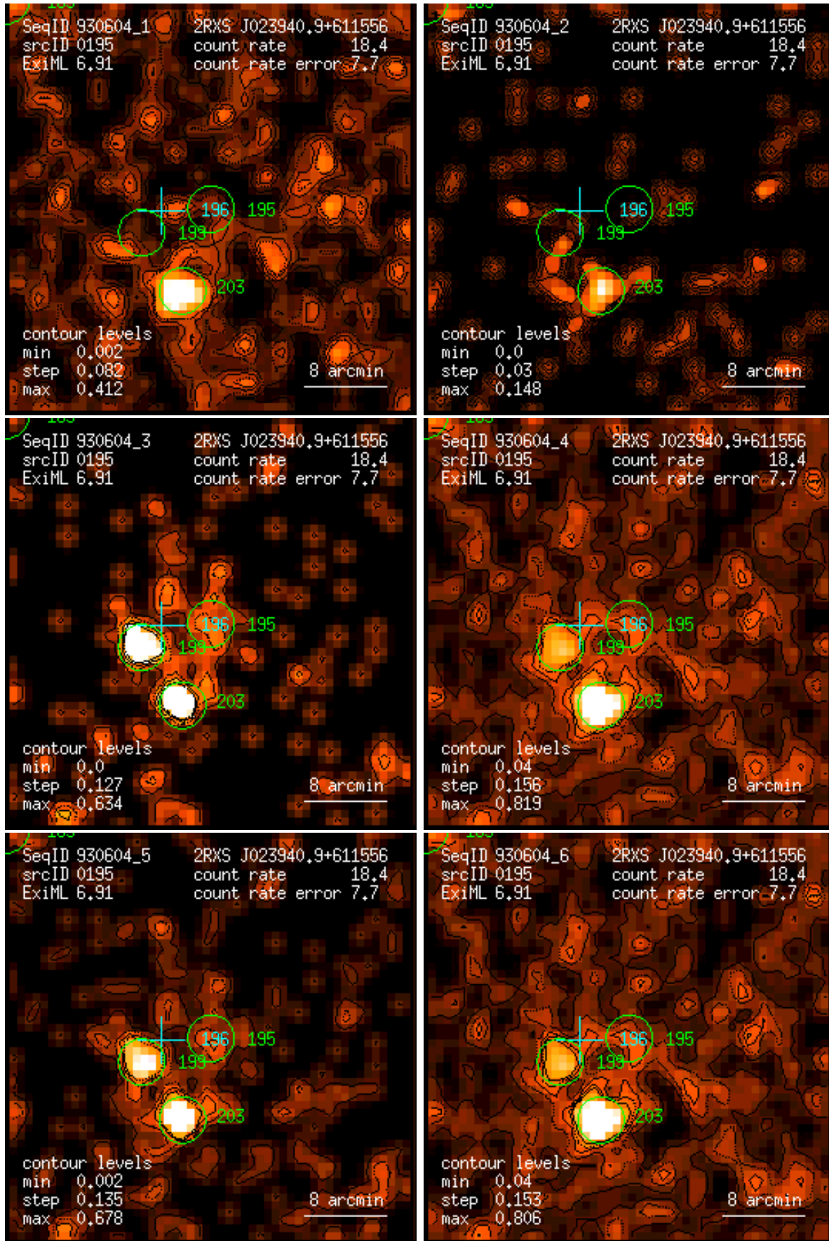
Figure 195: RASS 930604: detection 0195: band rate images, Gaussian filter: (1) PSPC channels 11 – 41, (2) 52 – 90, (3) 91 – 201, (4) 11 – 235, (5) 52 – 201, (6) 11 – 201. Broad band rates in counts/ks. Band rate contour levels in counts/ks/arcmin 2 .
