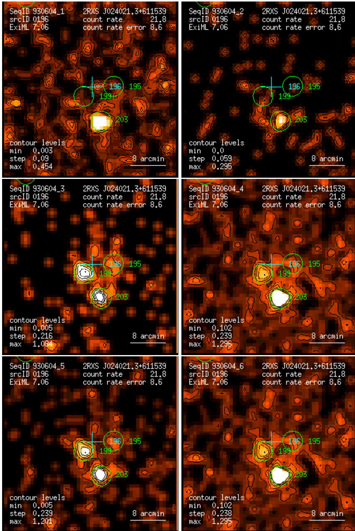
Figure 196: RASS 930604: detection 0196: band rate images, Gaussian filter: (1) PSPC channels 11 – 41, (2) 52 – 90, (3) 91 – 201, (4) 11 – 235, (5) 52 – 201, (6) 11 – 201. Broad band rates in counts/ks. Band rate contour levels in counts/ks/arcmin 2 .
