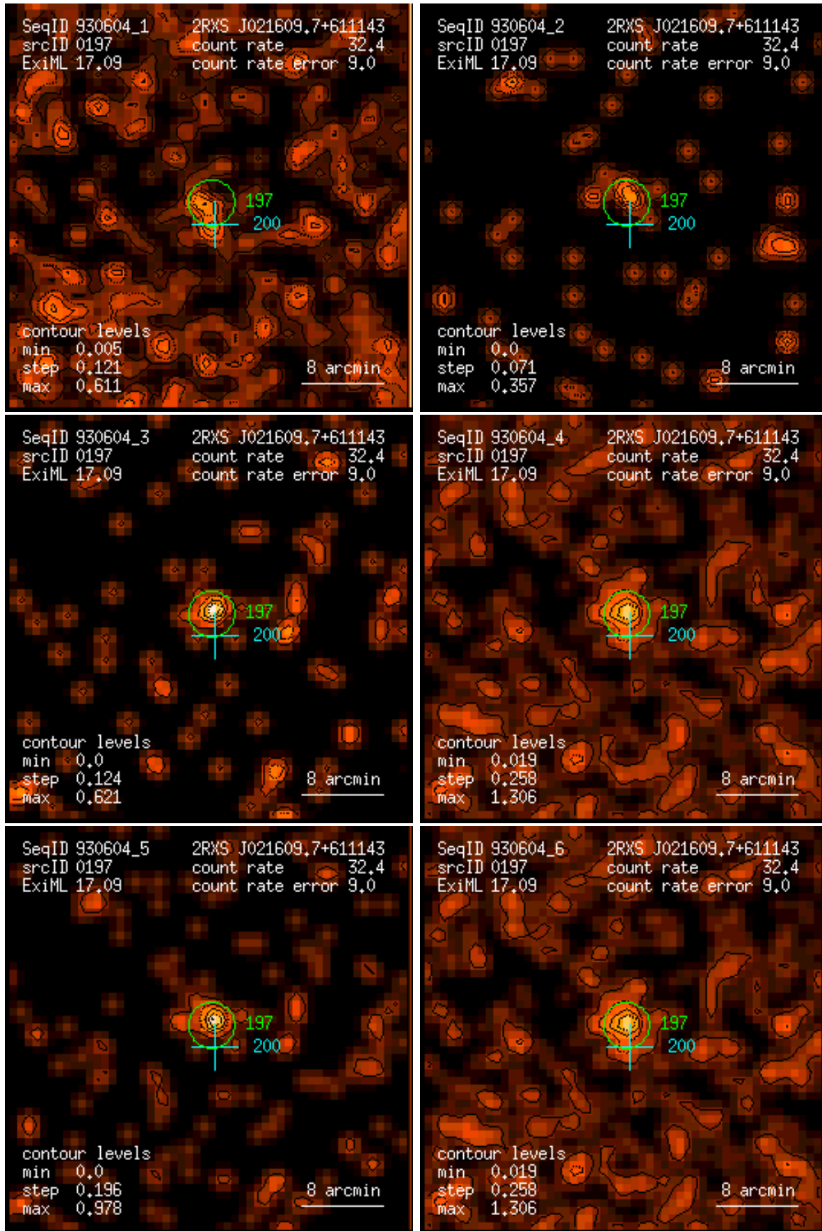
Figure 197: RASS 930604: detection 0197: band rate images, Gaussian filter: (1) PSPC channels 11 – 41, (2) 52 – 90, (3) 91 – 201, (4) 11 – 235, (5) 52 – 201, (6) 11 – 201. Broad band rates in counts/ks. Band rate contour levels in counts/ks/arcmin 2 .
