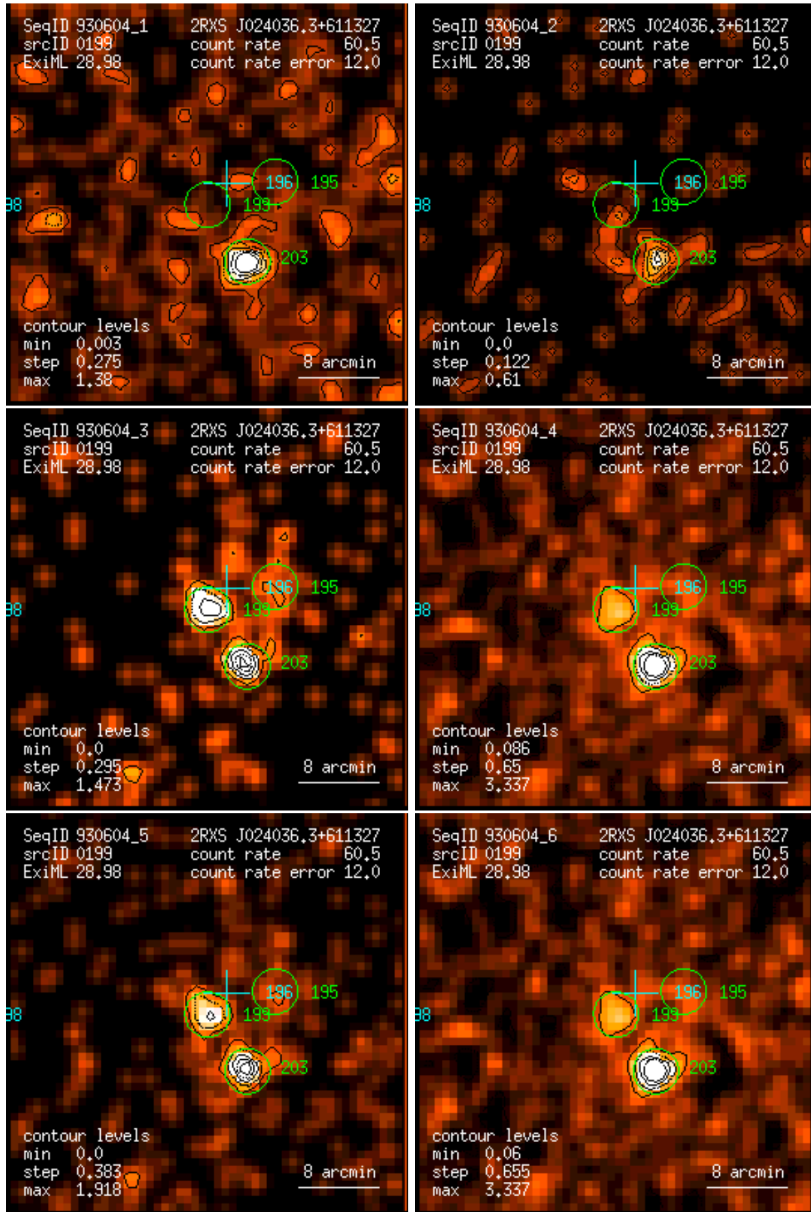
Figure 199: RASS 930604: detection 0199: band rate images, Gaussian filter: (1) PSPC channels 11 – 41, (2) 52 – 90, (3) 91 – 201, (4) 11 – 235, (5) 52 – 201, (6) 11 – 201. Broad band rates in counts/ks. Band rate contour levels in counts/ks/arcmin 2 .
