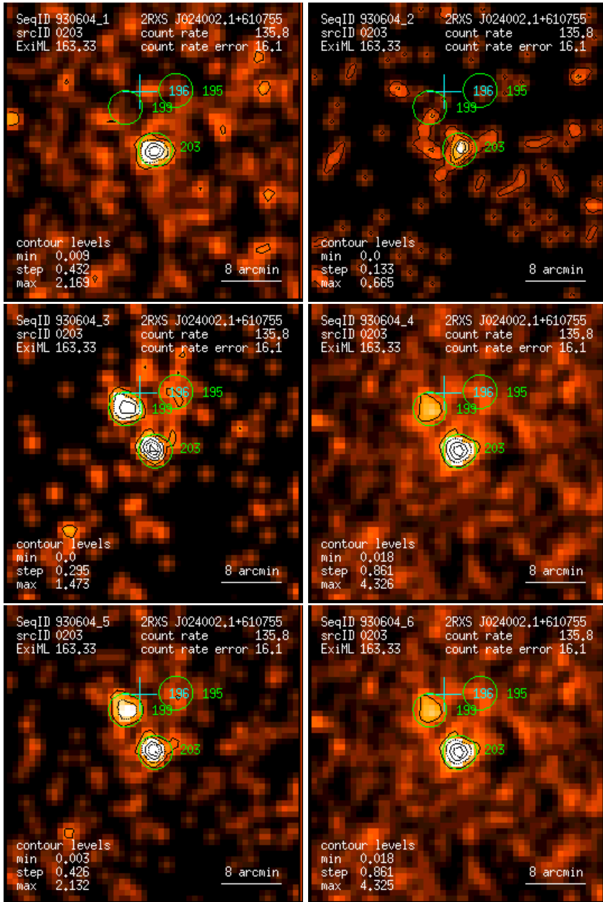
Figure 203: RASS 930604: detection 0203: band rate images, Gaussian filter: (1) PSPC channels 11 – 41, (2) 52 – 90, (3) 91 – 201, (4) 11 – 235, (5) 52 – 201, (6) 11 – 201. Broad band rates in counts/ks. Band rate contour levels in counts/ks/arcmin 2 .
