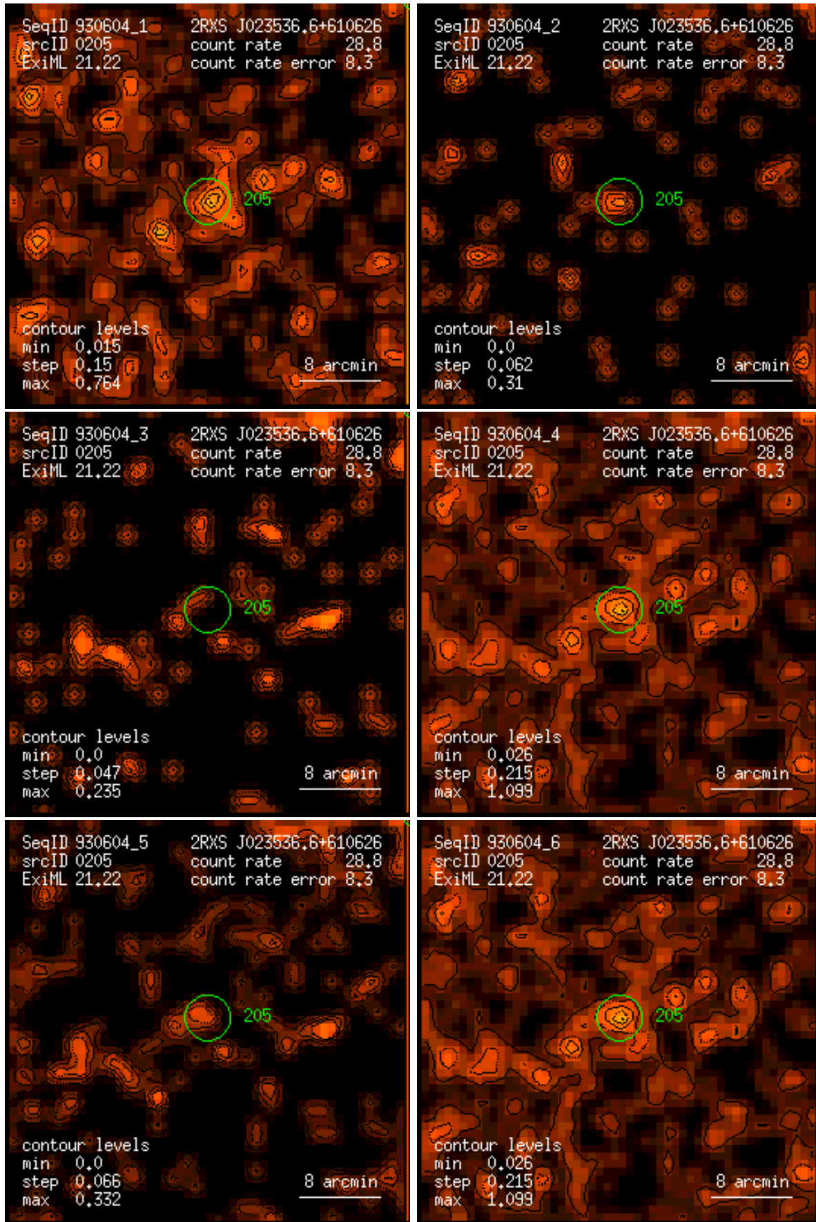
Figure 205: RASS 930604: detection 0205: band rate images, Gaussian filter: (1) PSPC channels 11 – 41, (2) 52 – 90, (3) 91 – 201, (4) 11 – 235, (5) 52 – 201, (6) 11 – 201. Broad band rates in counts/ks. Band rate contour levels in counts/ks/arcmin 2 .
