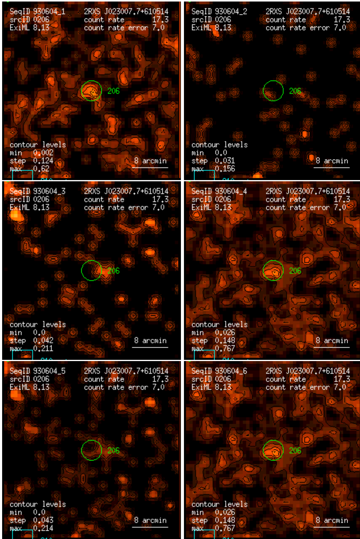
Figure 206: RASS 930604: detection 0206: band rate images, Gaussian filter: (1) PSPC channels 11 – 41, (2) 52 – 90, (3) 91 – 201, (4) 11 – 235, (5) 52 – 201, (6) 11 – 201. Broad band rates in counts/ks. Band rate contour levels in counts/ks/arcmin 2 .
