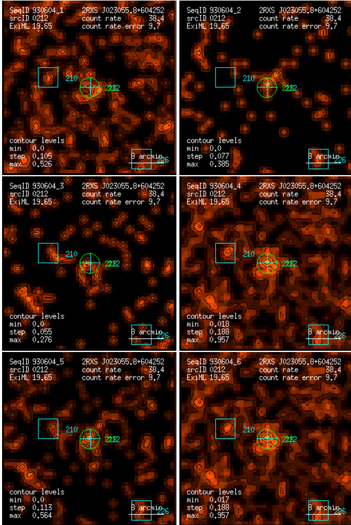
Figure 212: RASS 930604: detection 0212: band rate images, Gaussian filter: (1) PSPC channels 11 – 41, (2) 52 – 90, (3) 91 – 201, (4) 11 – 235, (5) 52 – 201, (6) 11 – 201. Broad band rates in counts/ks. Band rate contour levels in counts/ks/arcmin 2 .
