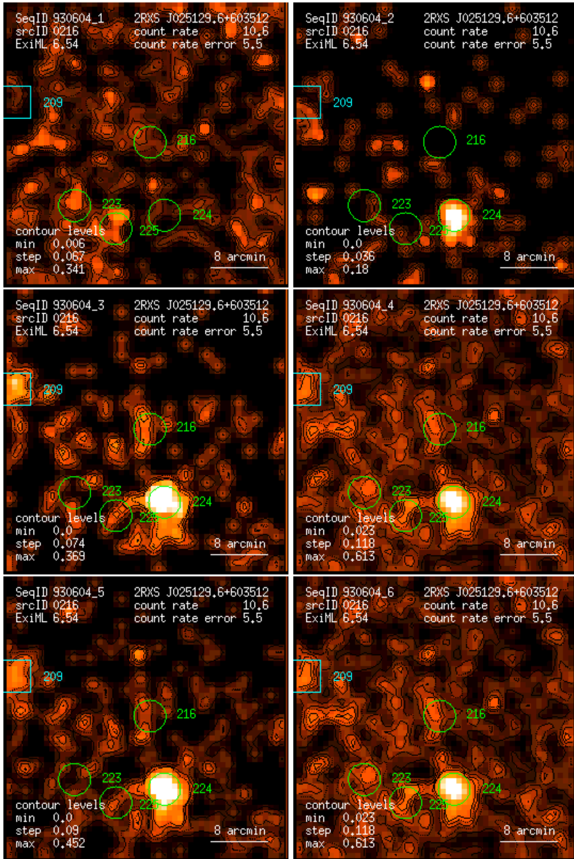
Figure 216: RASS 930604: detection 0216: band rate images, Gaussian filter: (1) PSPC channels 11 – 41, (2) 52 – 90, (3) 91 – 201, (4) 11 – 235, (5) 52 – 201, (6) 11 – 201. Broad band rates in counts/ks. Band rate contour levels in counts/ks/arcmin 2 .
