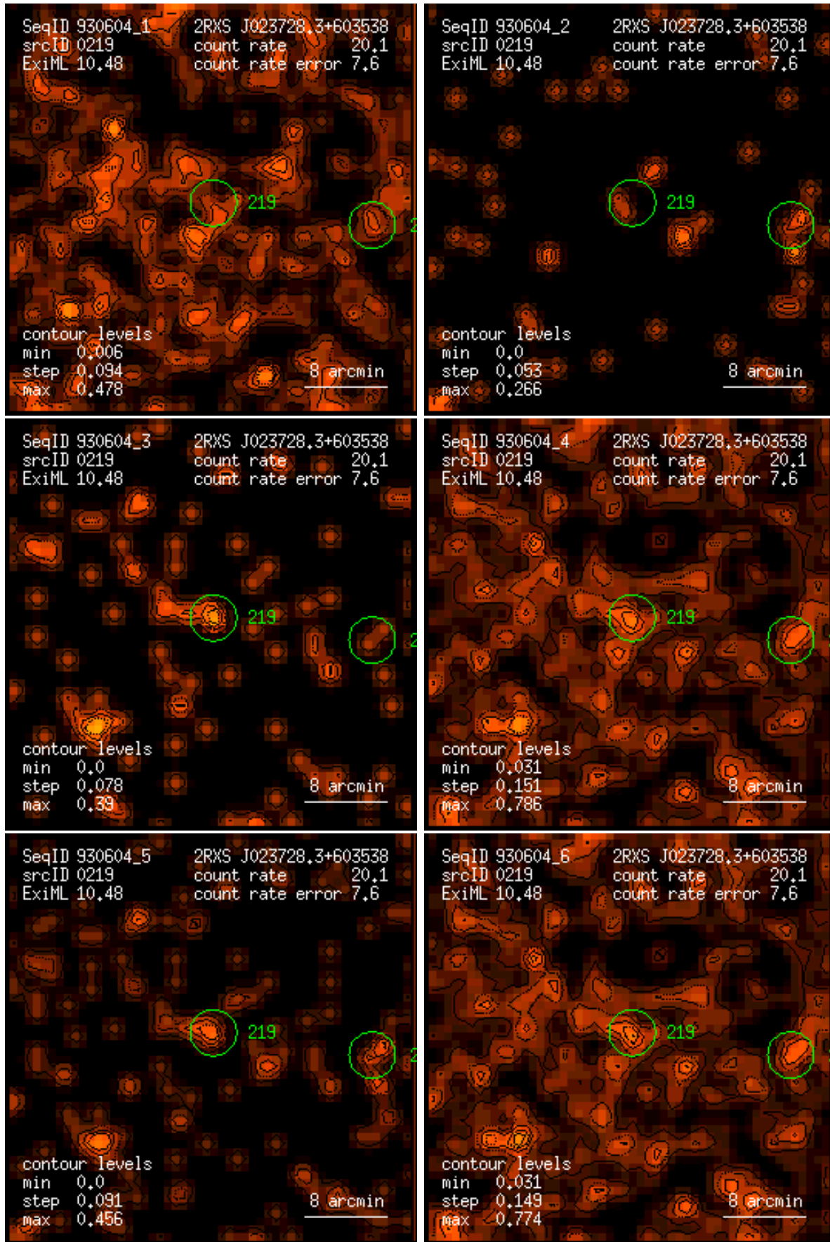
Figure 219: RASS 930604: detection 0219: band rate images, Gaussian filter: (1) PSPC channels 11 – 41, (2) 52 – 90, (3) 91 – 201, (4) 11 – 235, (5) 52 – 201, (6) 11 – 201. Broad band rates in counts/ks. Band rate contour levels in counts/ks/arcmin 2 .
