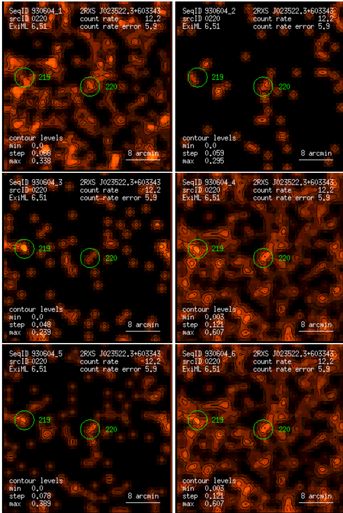
Figure 220: RASS 930604: detection 0220: band rate images, Gaussian filter: (1) PSPC channels 11 – 41, (2) 52 – 90, (3) 91 – 201, (4) 11 – 235, (5) 52 – 201, (6) 11 – 201. Broad band rates in counts/ks. Band rate contour levels in counts/ks/arcmin 2 .
