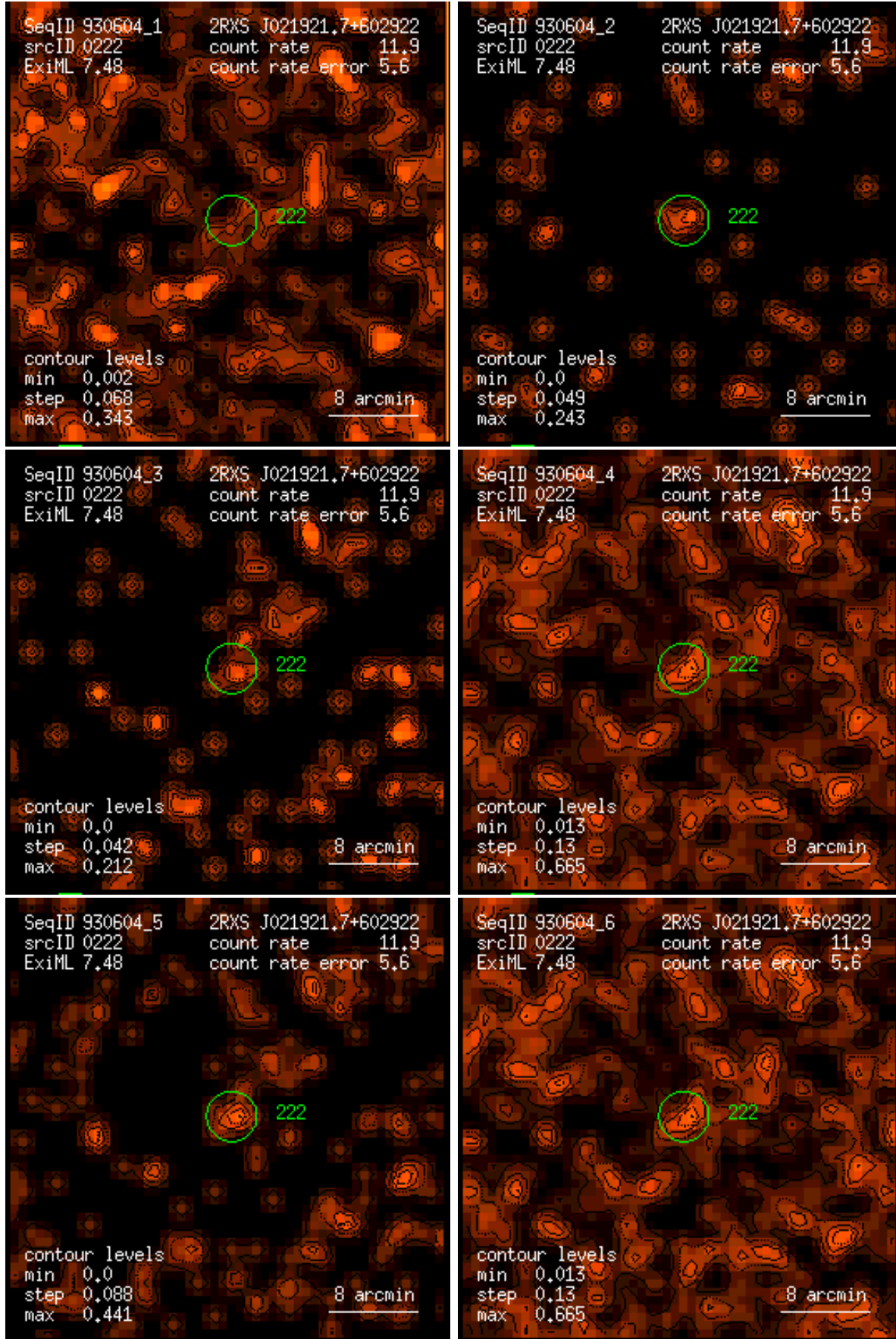
Figure 222: RASS 930604: detection 0222: band rate images, Gaussian filter: (1) PSPC channels 11 – 41, (2) 52 – 90, (3) 91 – 201, (4) 11 – 235, (5) 52 – 201, (6) 11 – 201. Broad band rates in counts/ks. Band rate contour levels in counts/ks/arcmin 2 .
