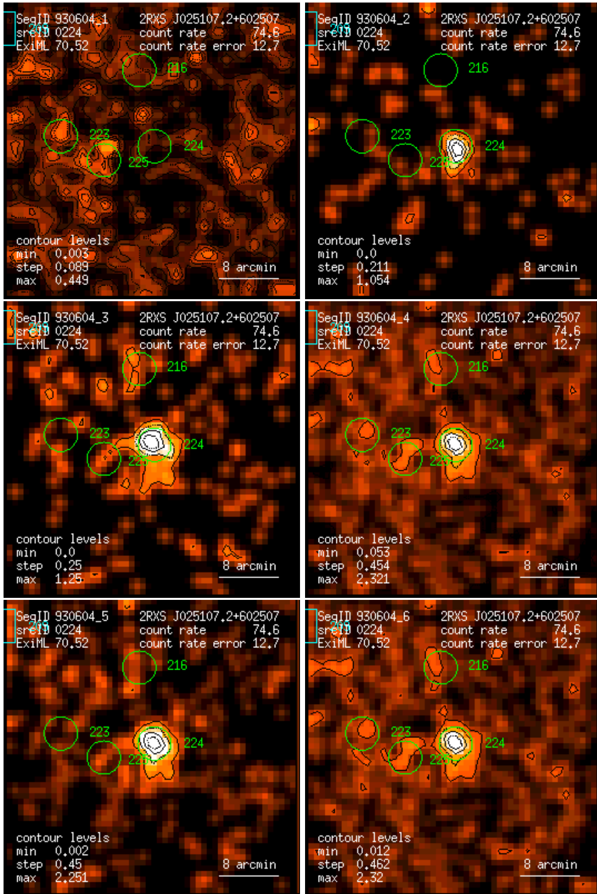
Figure 224: RASS 930604: detection 0224: band rate images, Gaussian filter: (1) PSPC channels 11 – 41, (2) 52 – 90, (3) 91 – 201, (4) 11 – 235, (5) 52 – 201, (6) 11 – 201. Broad band rates in counts/ks. Band rate contour levels in counts/ks/arcmin 2 .
