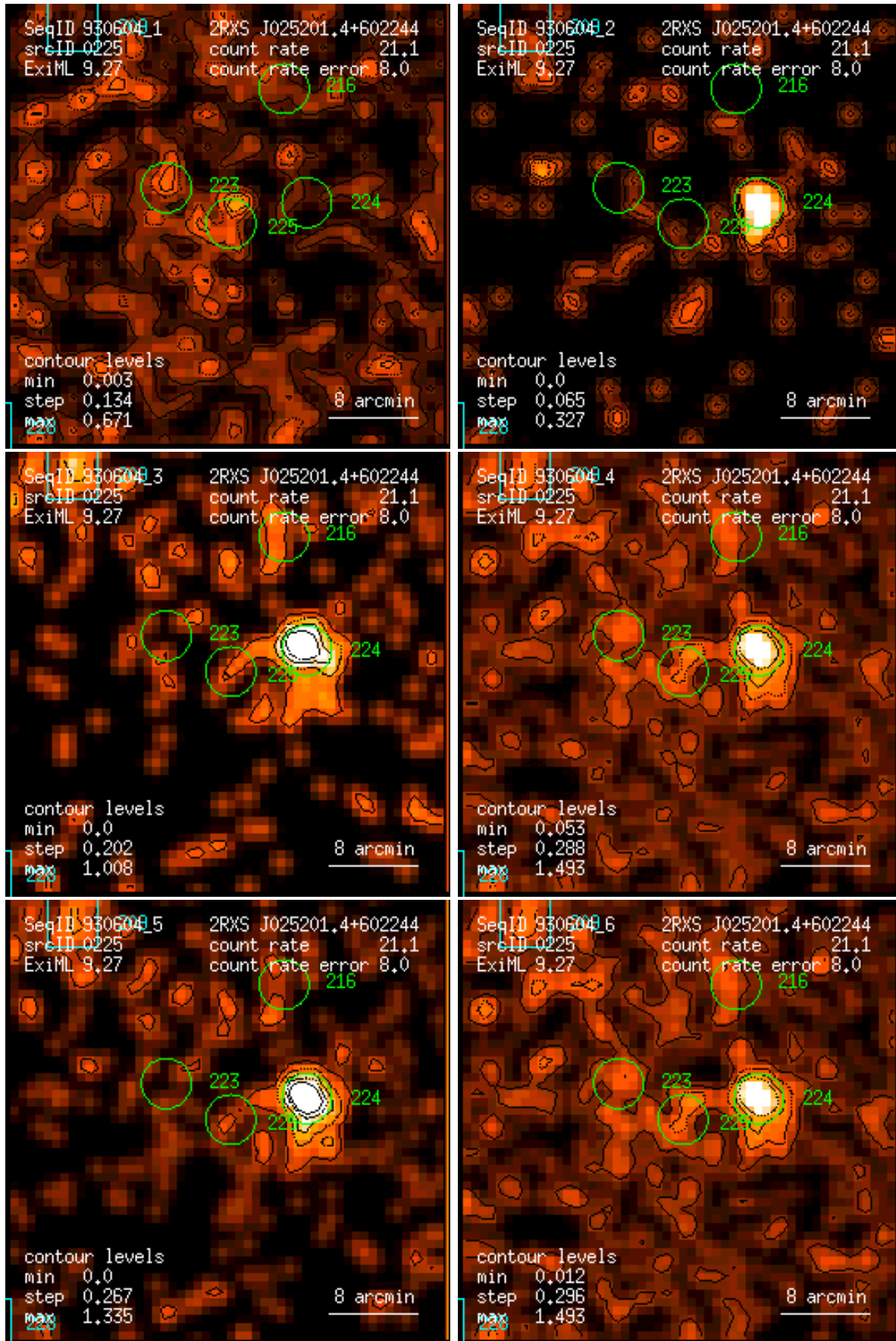
Figure 225: RASS 930604: detection 0225: band rate images, Gaussian filter: (1) PSPC channels 11 – 41, (2) 52 – 90, (3) 91 – 201, (4) 11 – 235, (5) 52 – 201, (6) 11 – 201. Broad band rates in counts/ks. Band rate contour levels in counts/ks/arcmin 2 .
